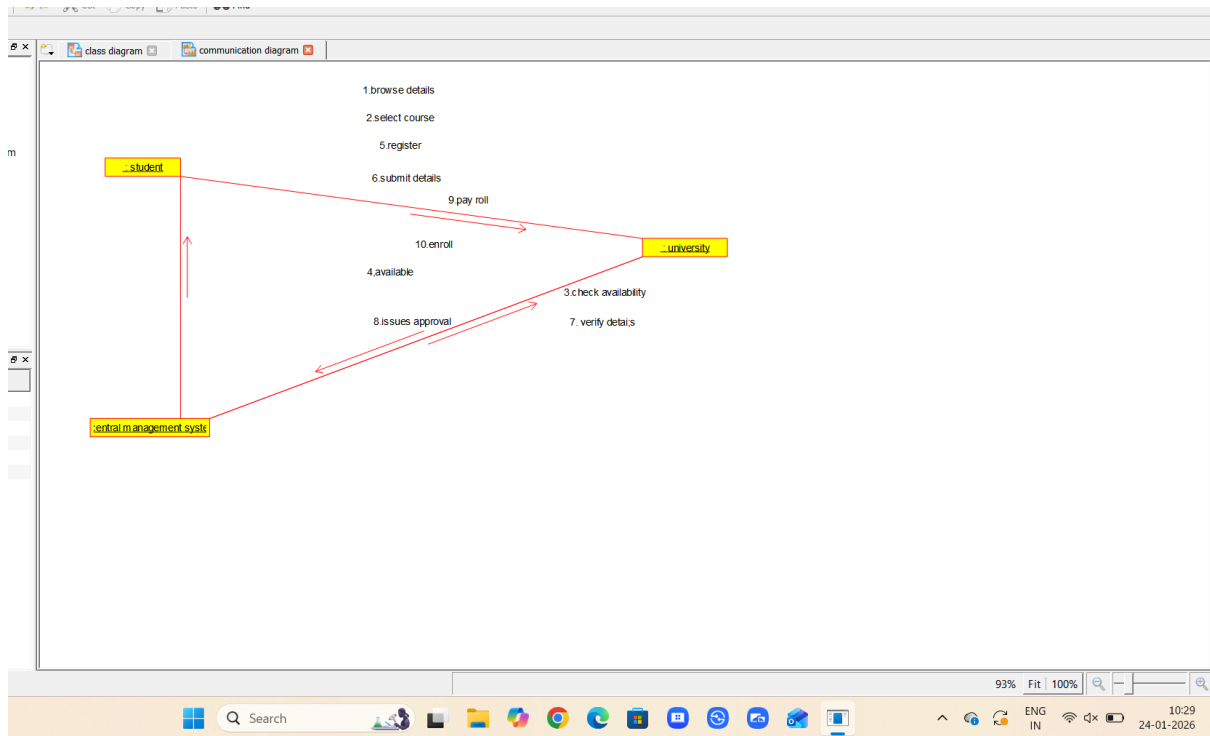
COLLABORATION DIAGRAM
