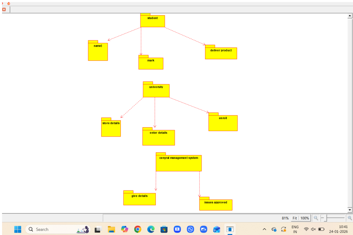
PACKAGE DIAGRAM
