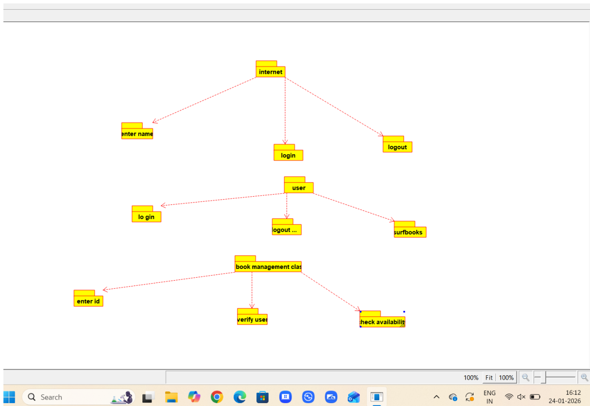
PACKAGE DIAGRAM
