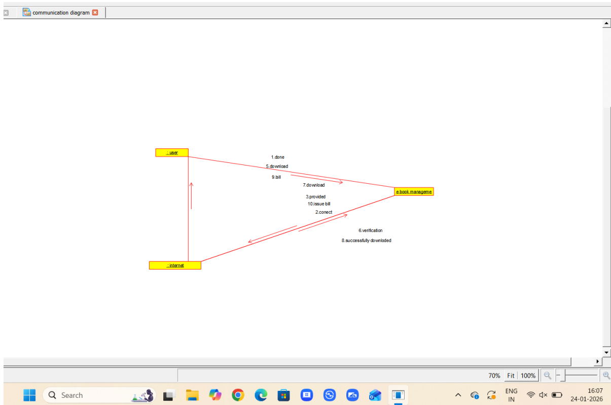
COLLABORATION DIAGRAM
