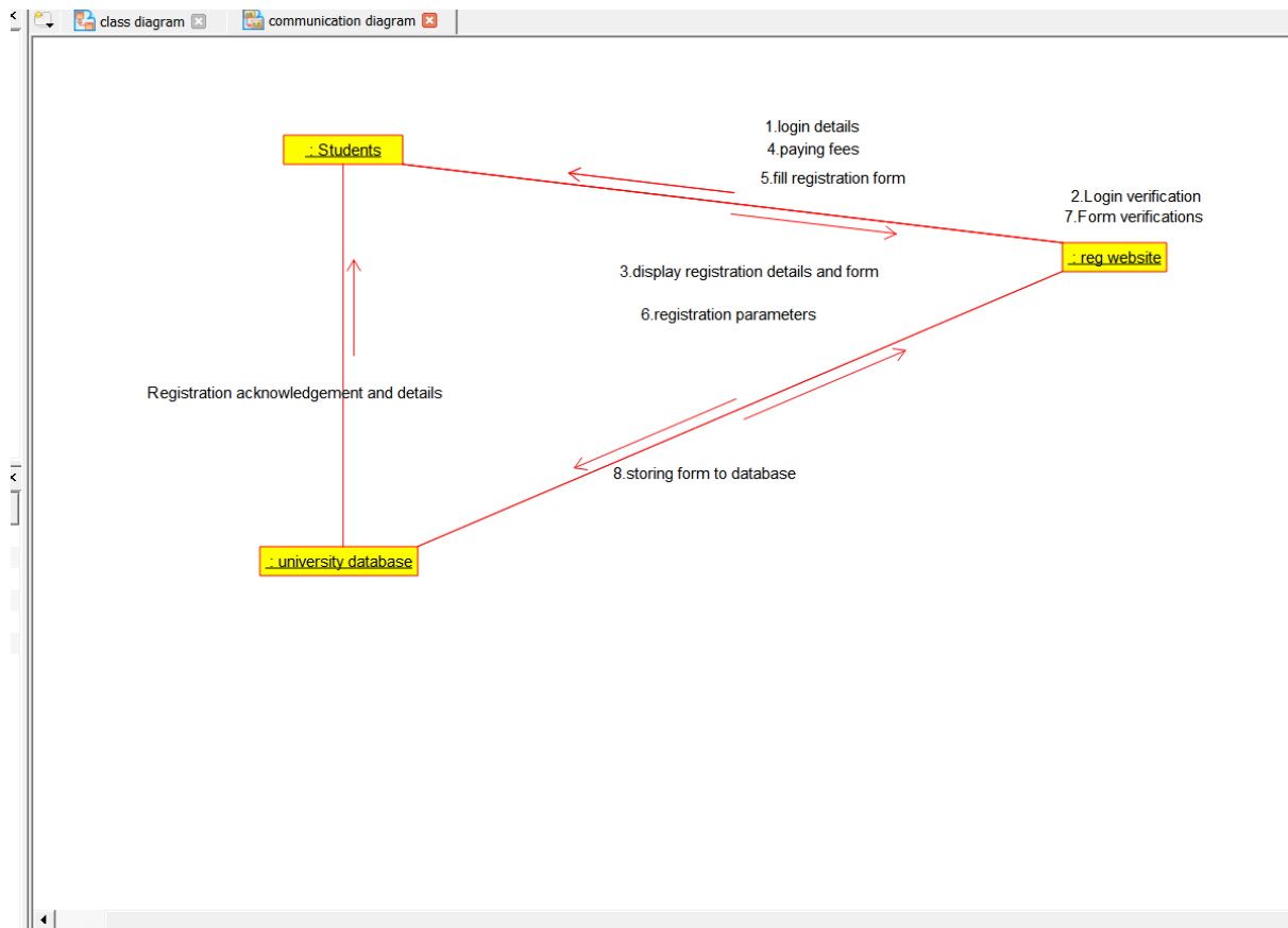
COLLABORATION DIAGRAM
