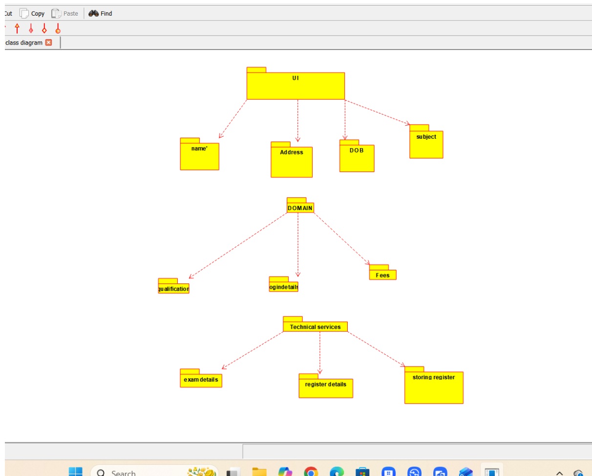
PACKAGE DIAGRAM
