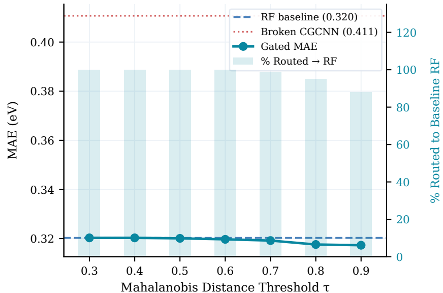
Gating Sweep — Band Gap
