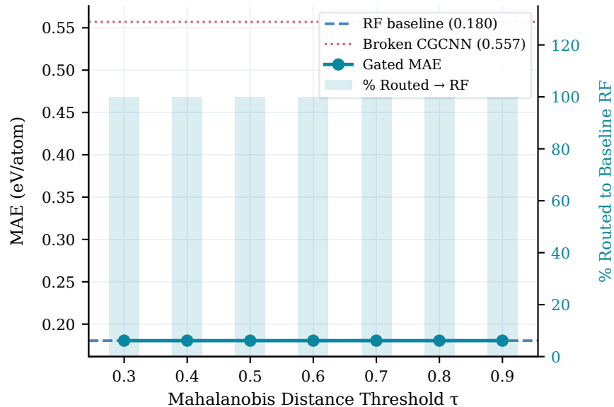
Gating Sweep — Formation Energy
