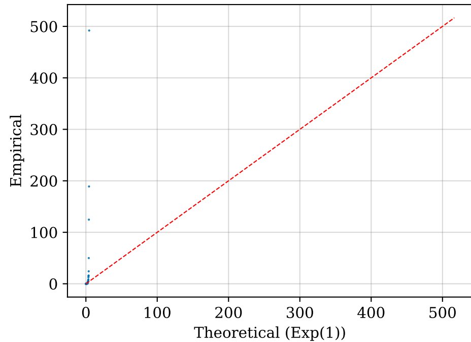
QQ — BTC Rescaled Inter-arrivals
