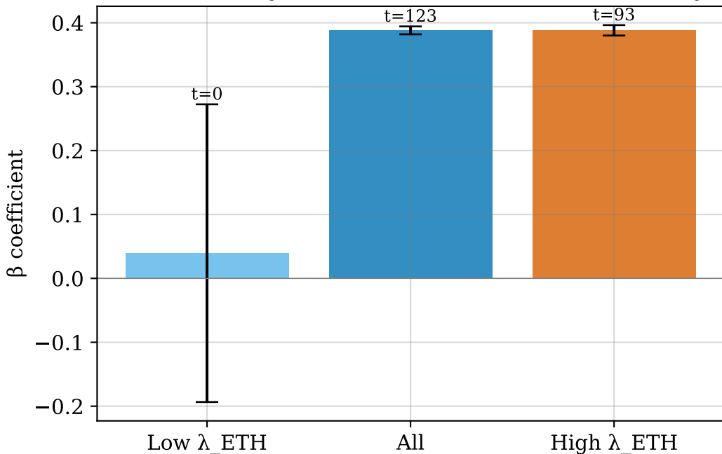
Predictability Conditioned on Hawkes Intensity
