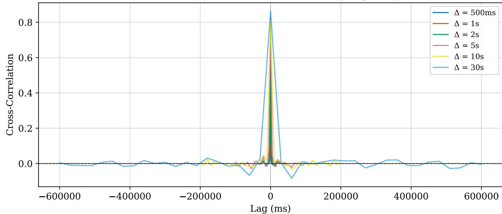
Cross-Correlation Function at Various Sampling Frequencies
