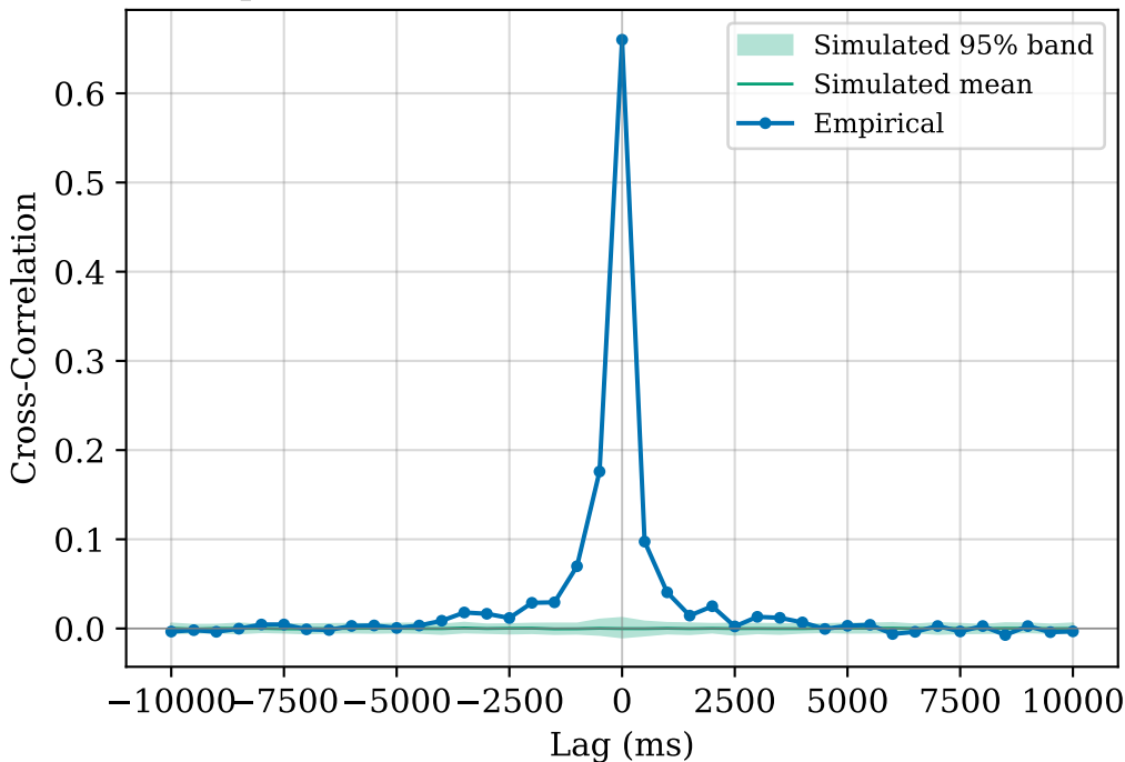
Empirical vs Simulated CCF (Hawkes Model)
