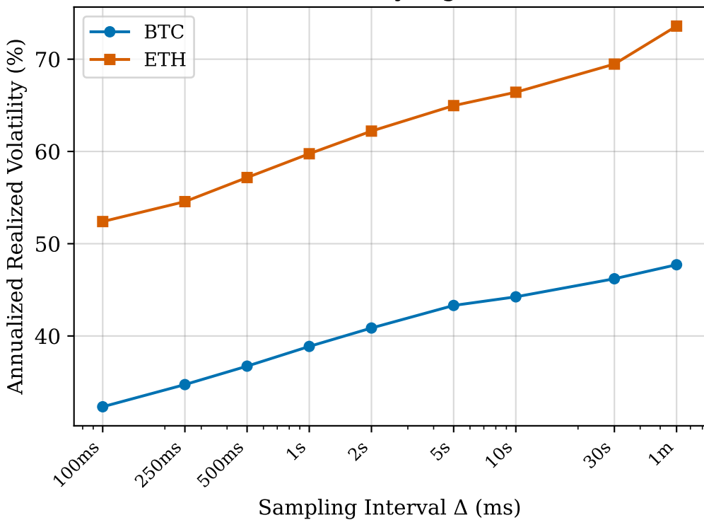
Realized Volatility Signature Plot
