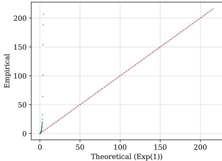
QQ — ETH Rescaled Inter-arrivals
