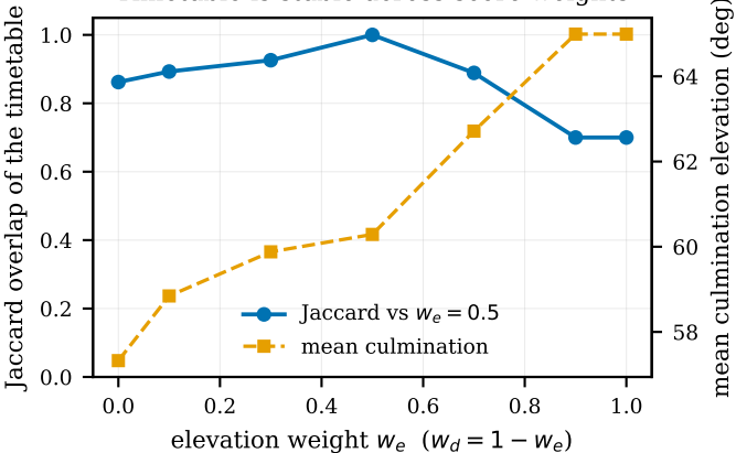
Timetable is stable across score weights
