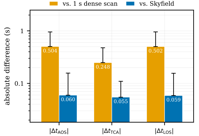
Fig. 3. Pass-timing agreement against both references. Bars are means and caps the 95th percentile; note the logarithmic axis, since the two references differ by roughly an order of magnitude. The larger apparent deviation from the 1 s dense scan reflects that reference’s own grid quantisation, not error in the refined estimator.
