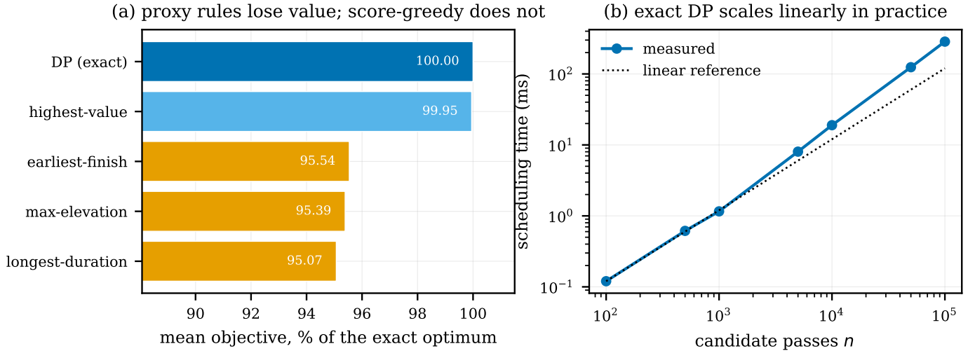
Fig. 11. (a) Greedy heuristics leave value on the table against the exact dynamic program. (b) Scheduling time grows linearly in practice, remaining negligible at catalogue scale.
