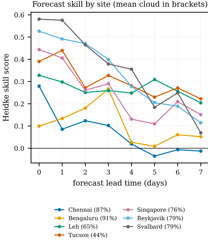
Fig. 5. Forecast skill against lead time, per station. The spread between stations is as large as the decay with lead time, so a planner’s expected benefit from weather-awareness is a local property, not a universal constant.
