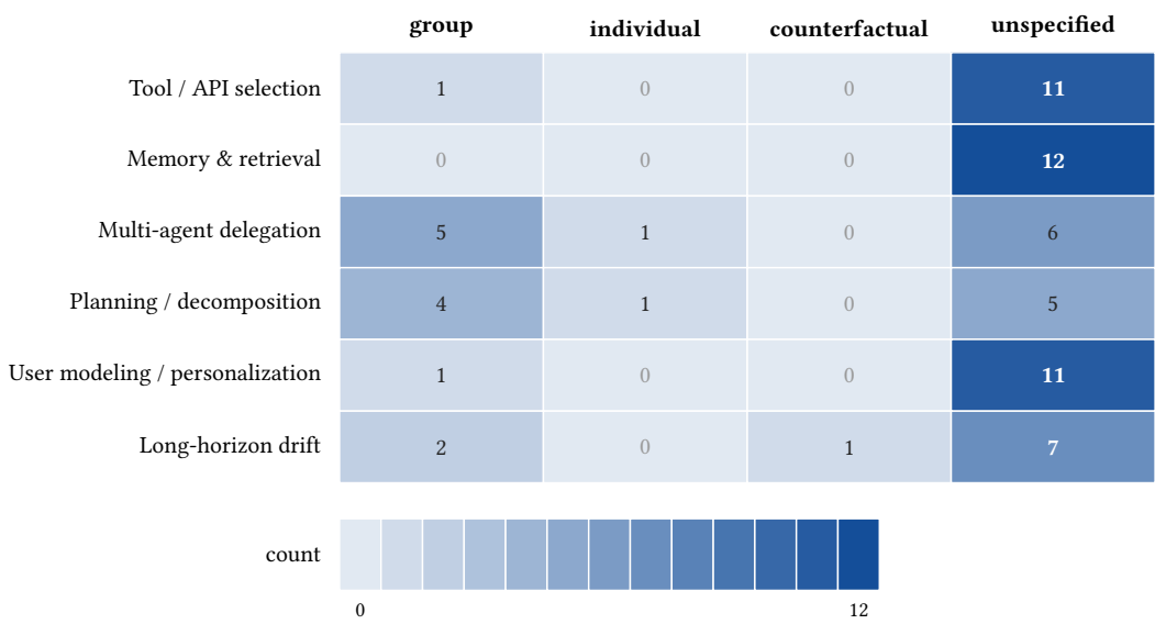
Fig. 4. Coverage matrix (agent component \times fairness dimension), cells shaded by paper count (single-hue, colorblind-safe blue). The counterfactual column holds exactly one nonzero cell (long-horizon drift, [? ]); the unspecified column dominates with 52 of 68 component-branch entries.
