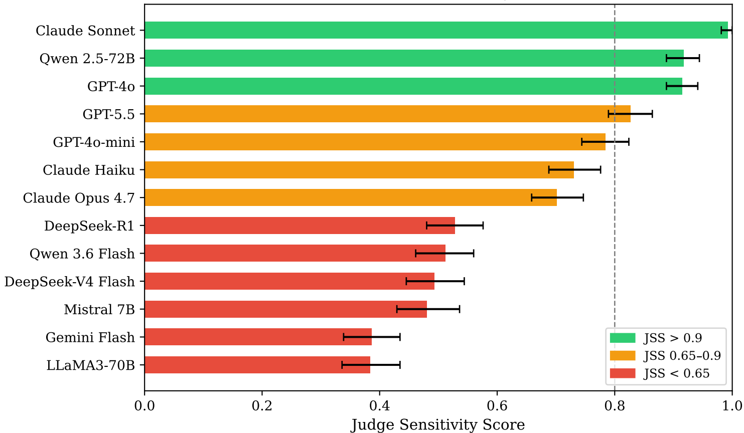
Coherence Task: JSS by Model
