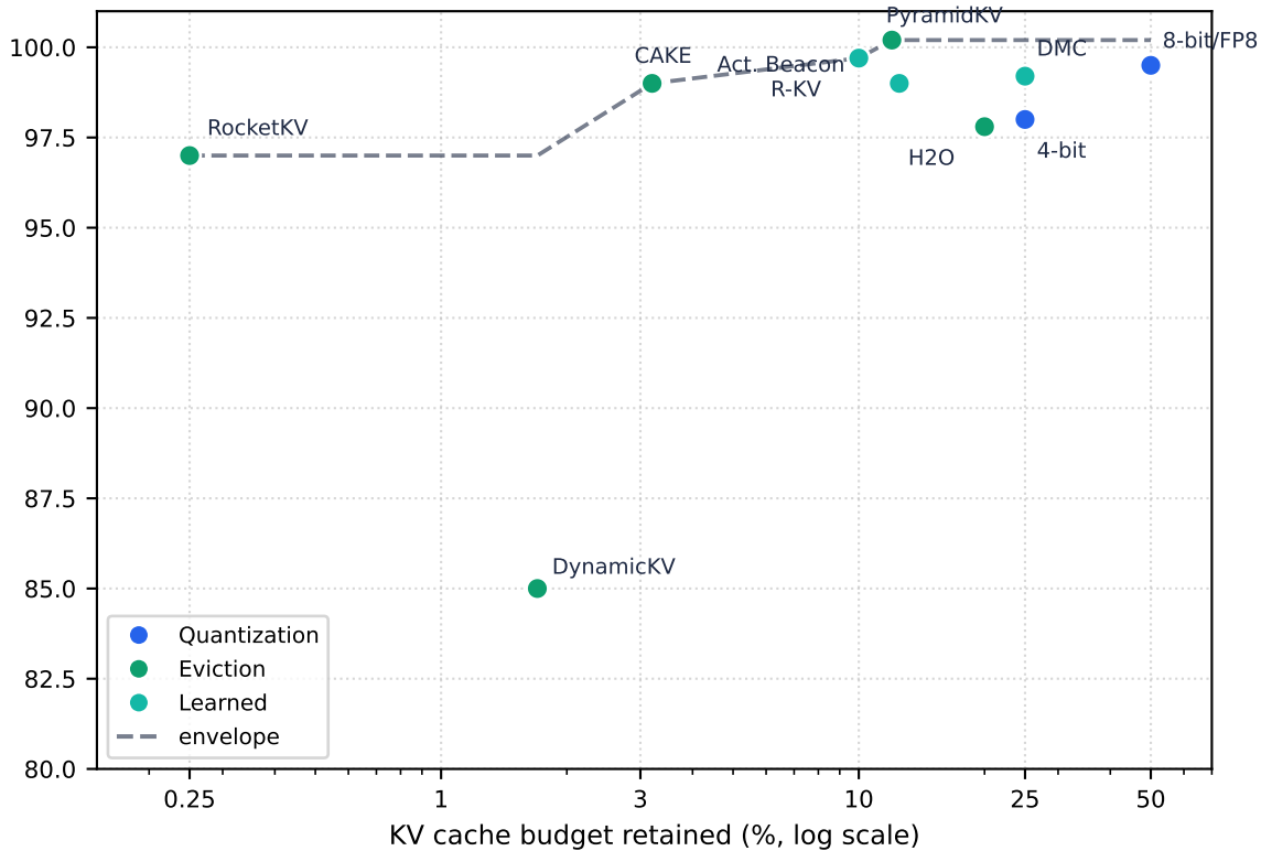
Reported accuracy retention (%)
