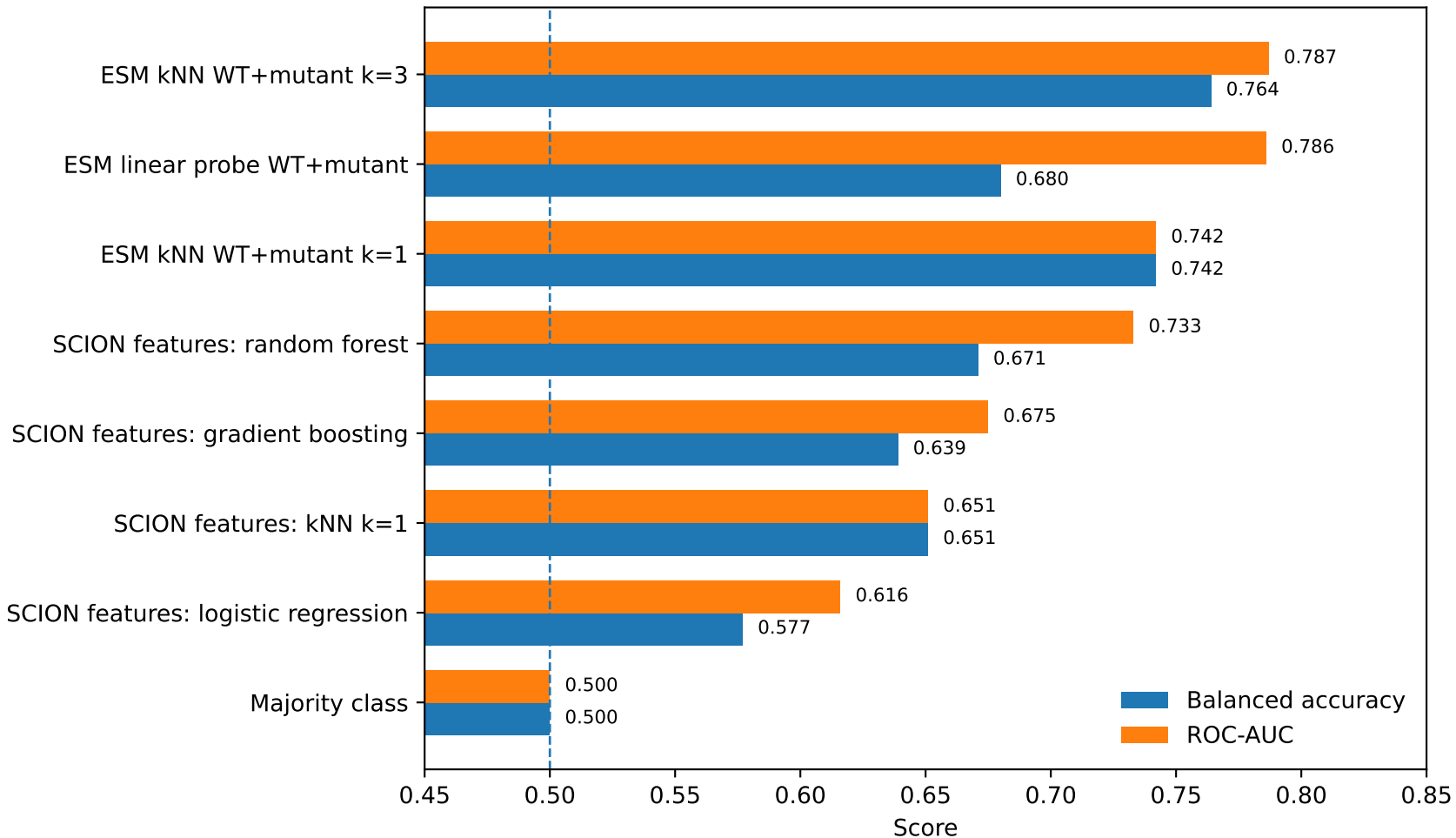
Held-out SCN1A GoF/LoF prediction
