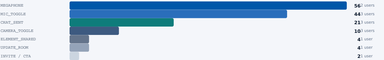
ACTION MIX (all 3 interactive users combined)
