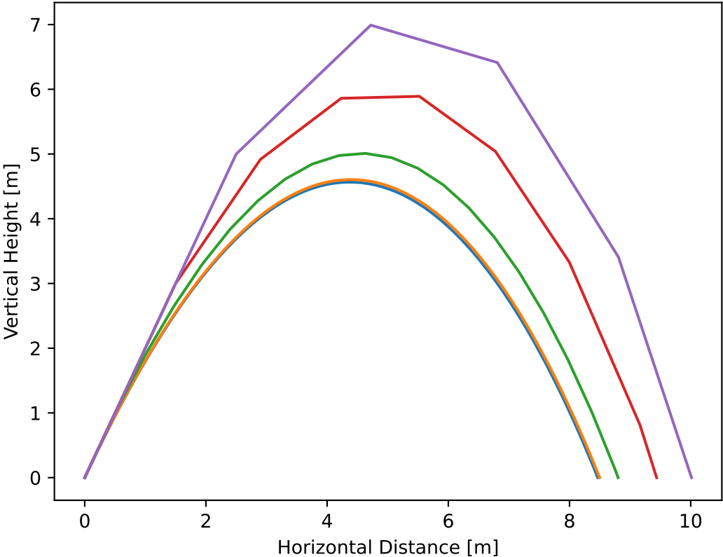
Projectile Motion with quadratic drag using Euler's Method with different step sizes
