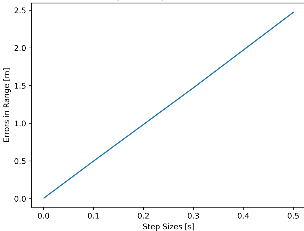
Errors in Range vs. Step Sizes for Euler's Method
