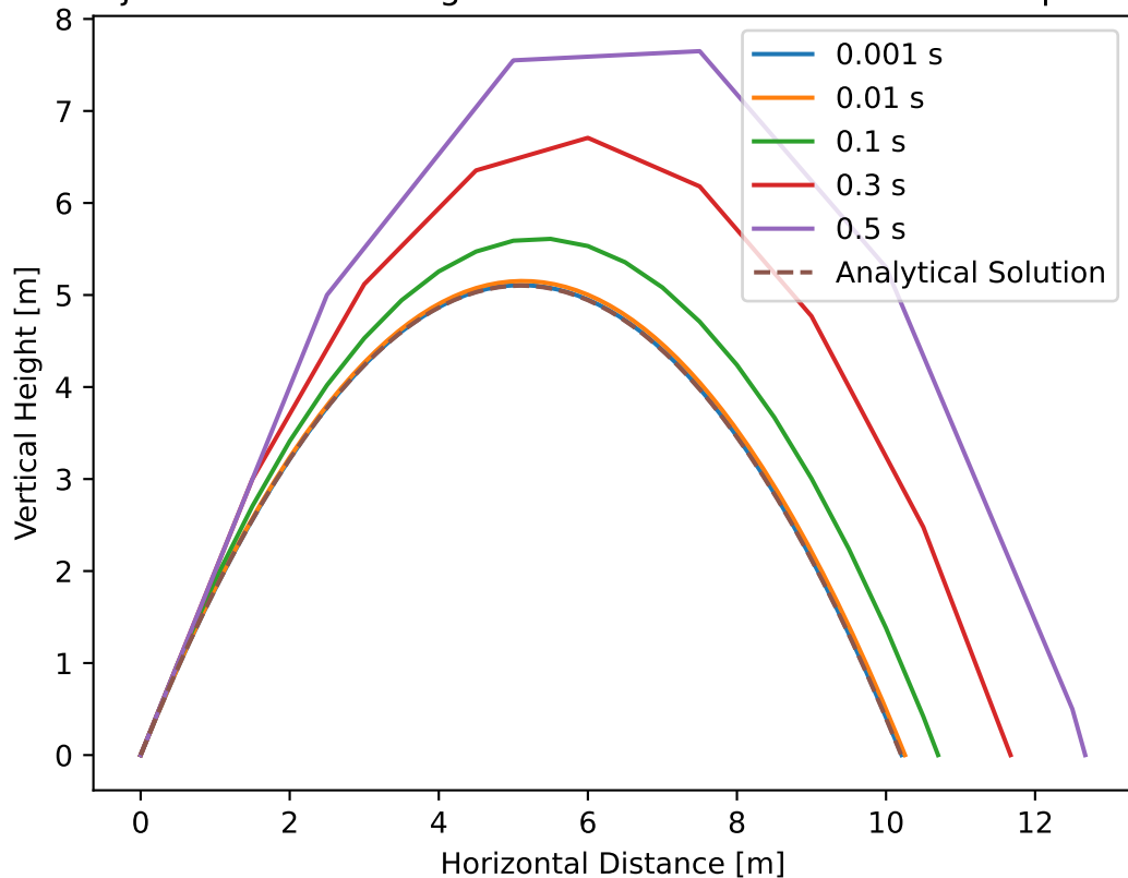
Projectile Motion using Euler's Method with different step sizes
