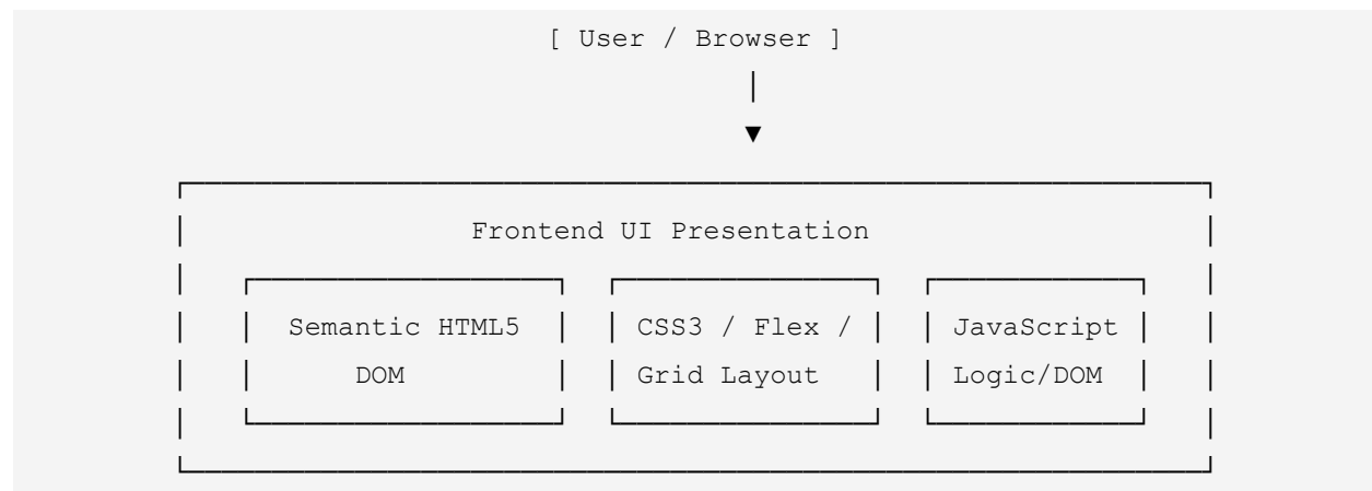
Figure 4.1: High-level architectural structure of the Frontend Web Application
