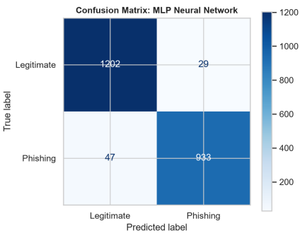
Figure 7c: CM — MLP Neural Network
