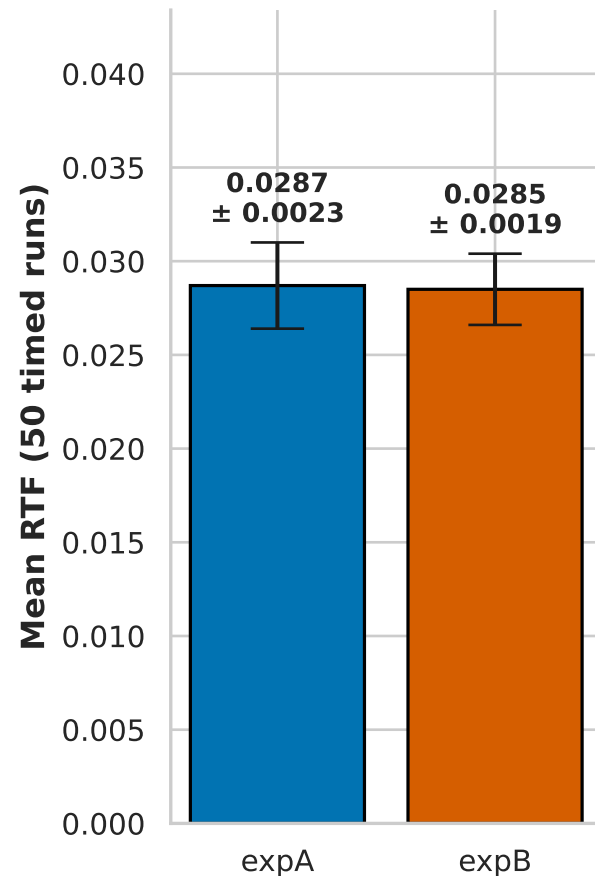
Overall RTF mean \pm stdev
