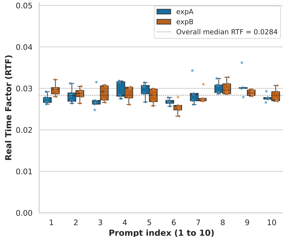
Per-prompt RTF distribution (5 timed runs each) Lower is faster, RTF < 1.0 means faster than real time
