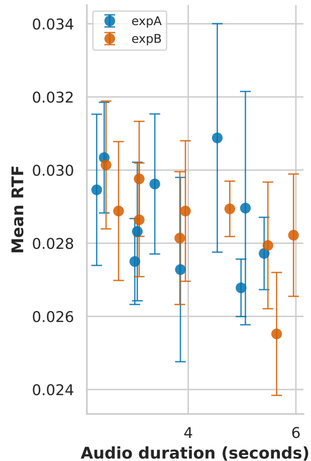
RTF vs audio duration
