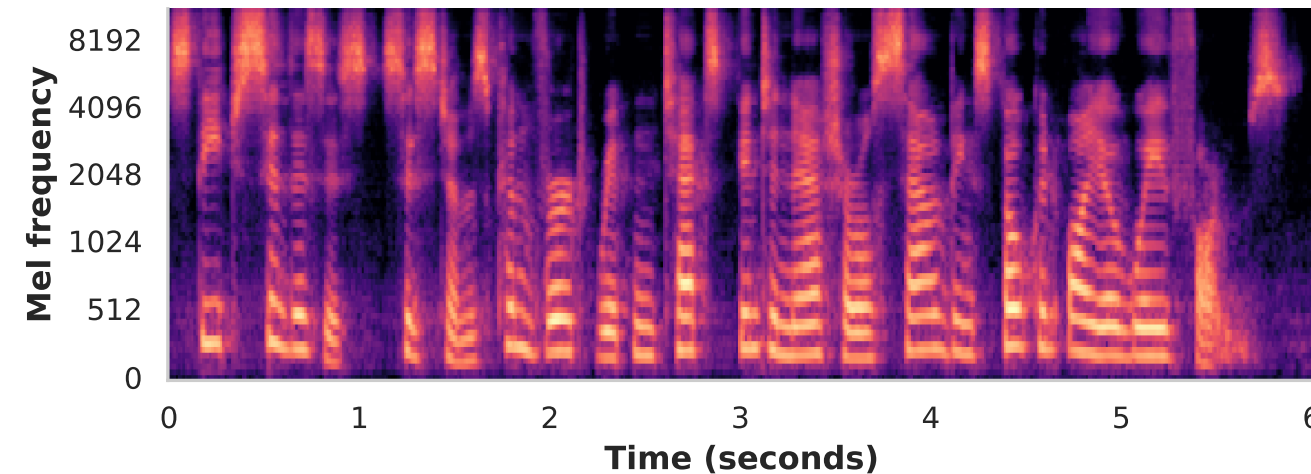
expB sample 10: "Speech synthesis systems convert written text into natu..."
