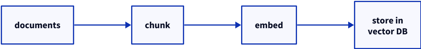
Indexing pipeline: documents to chunk to embed to store in vector DB
