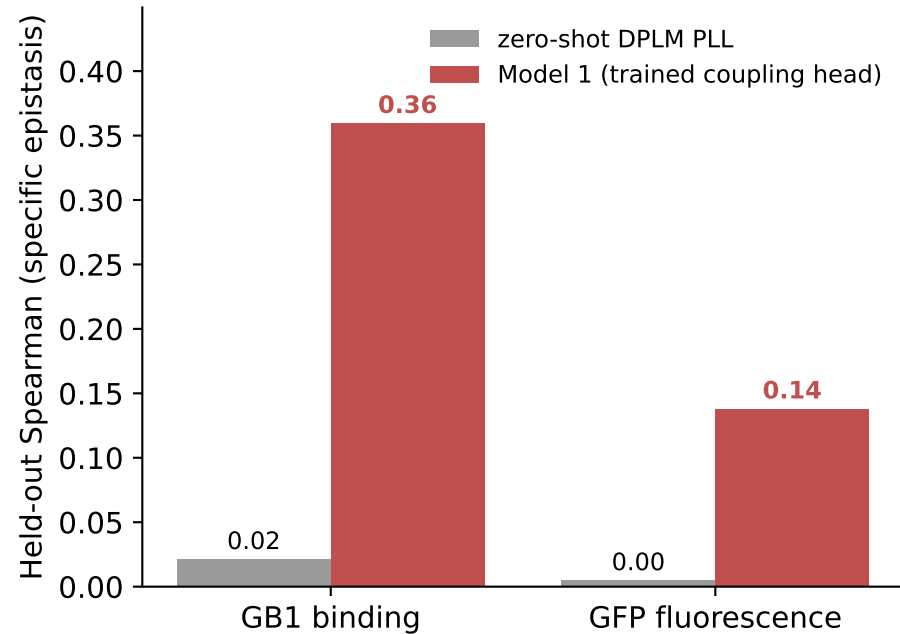
A Model 1 predicts functional epistasis; zero-shot DPLM cannot
