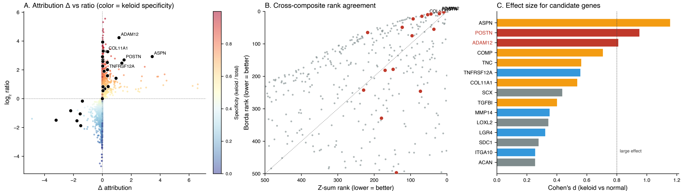
Figure 4 — Cross-metric validation of foundation-model gene rankings
