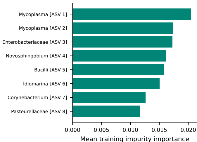
c Exploratory microbial ranks
