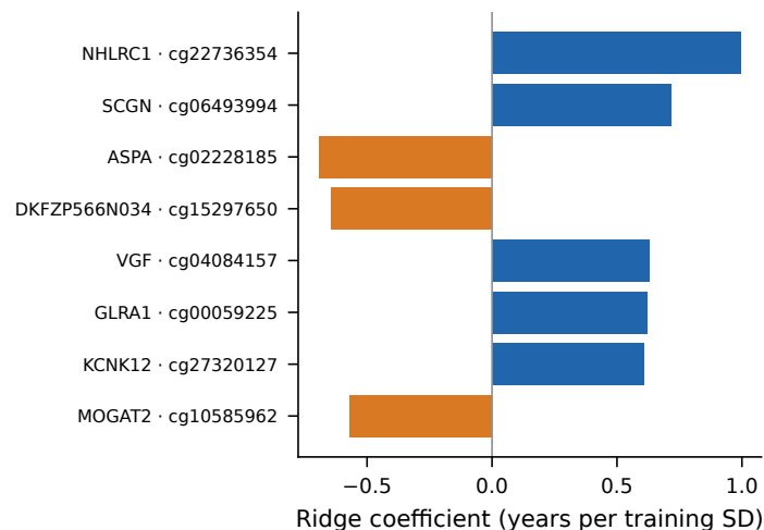
d Label-shuffle controls
