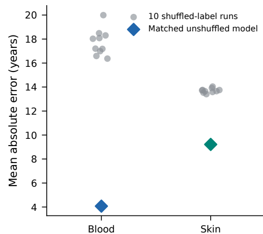
d Label-shuffle controls
