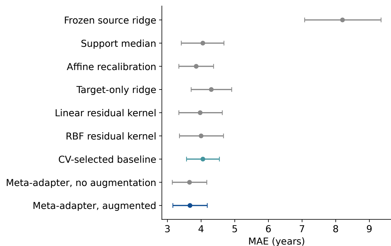
f 16-shot neural prediction calibration
