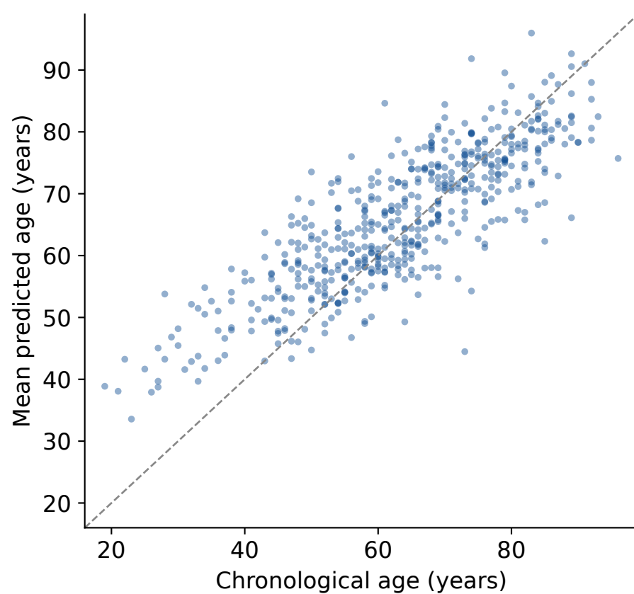
e 16-shot neural prediction calibration
