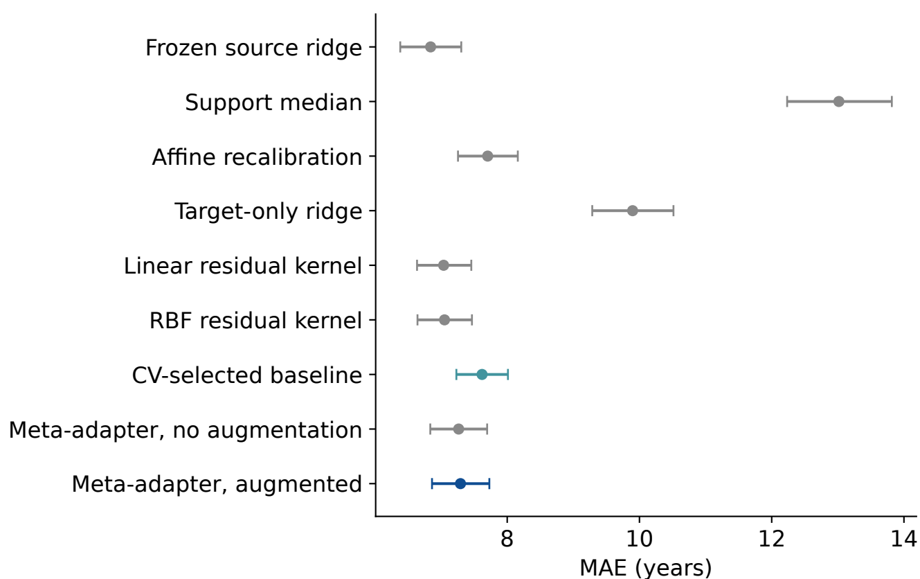
e 16-shot neural prediction calibration
