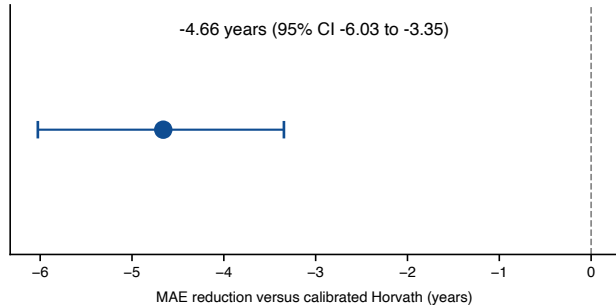
b Incremental microbial information
