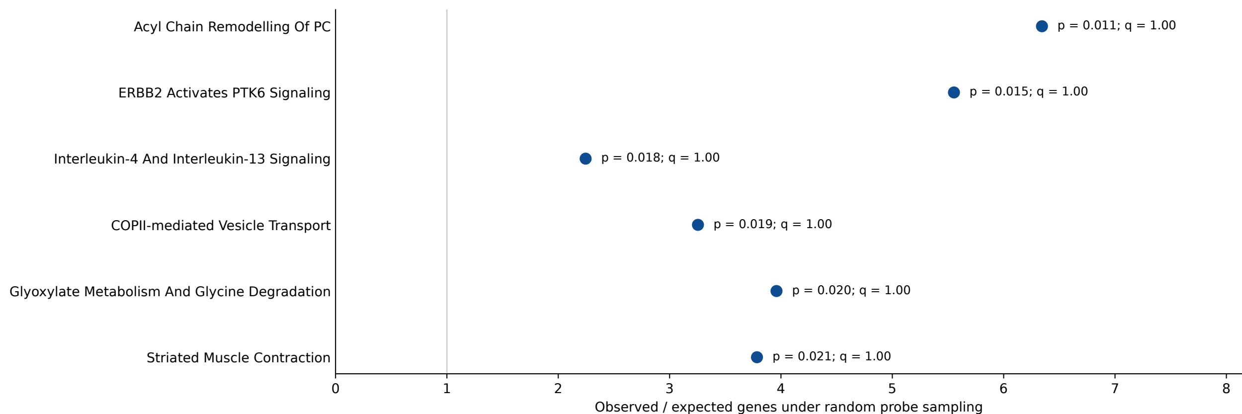
c Reactome annotation enrichment
