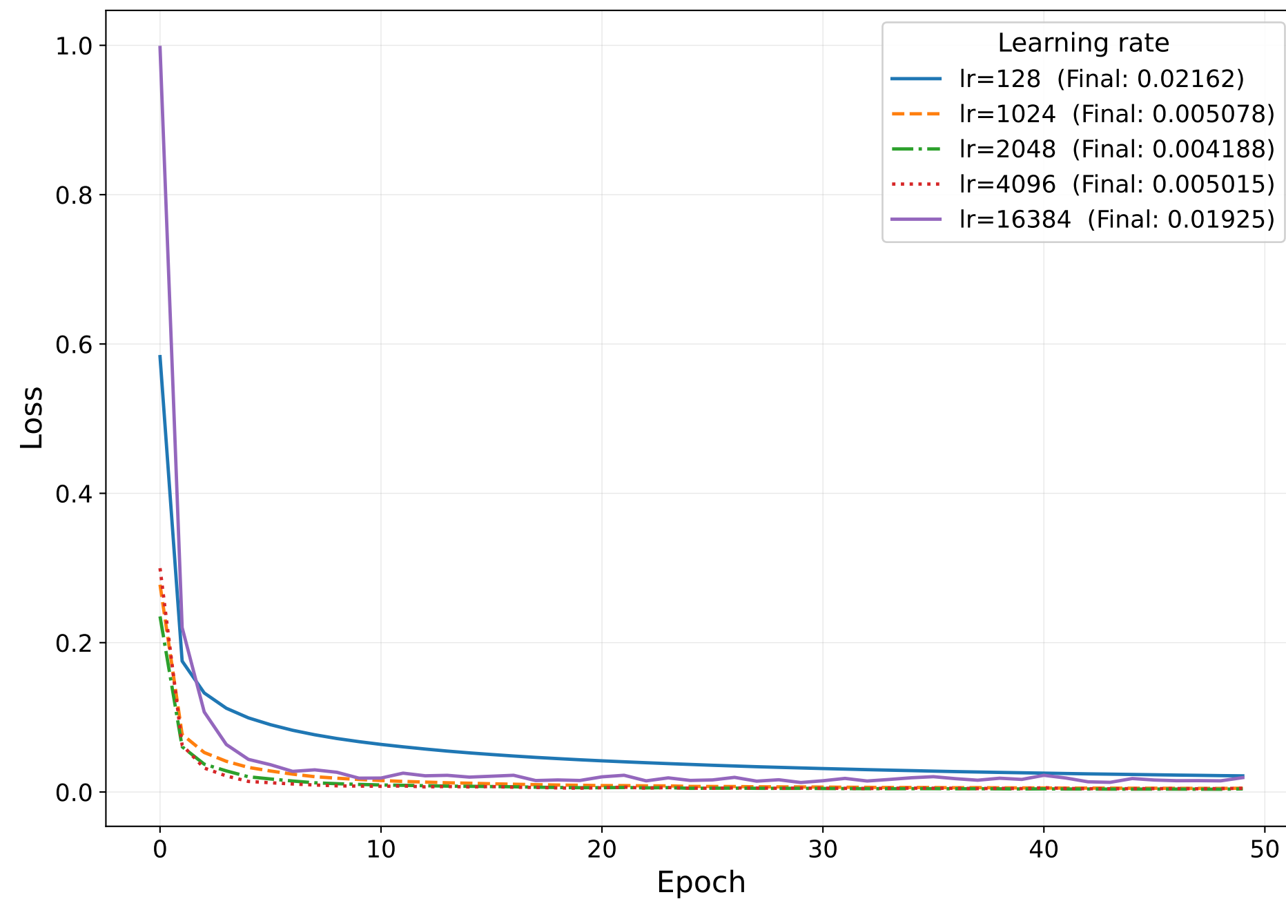
Batch size = 8192
