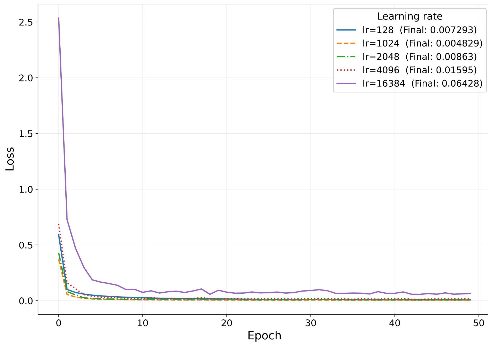
Batch size = 1024
