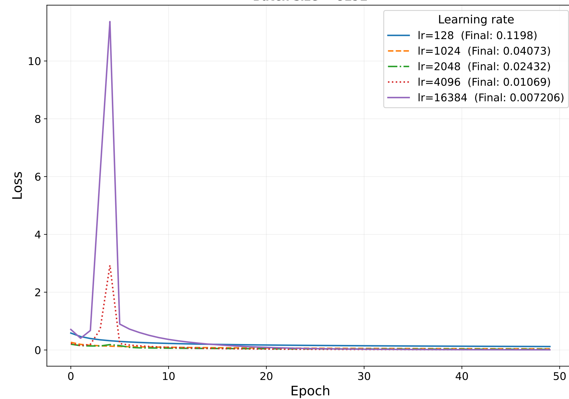
Batch size = 8192
