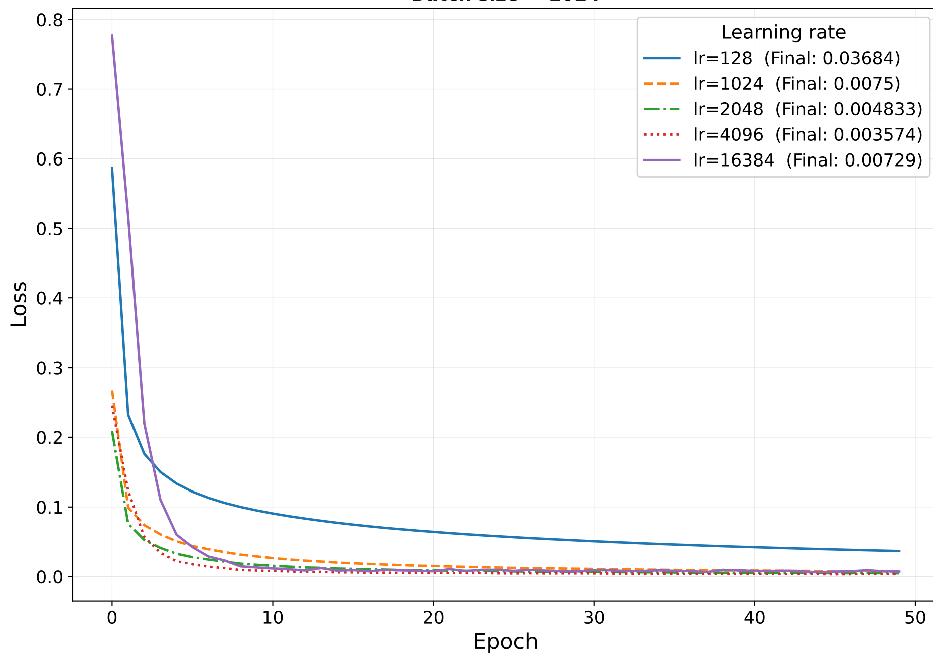
Batch size = 1024
