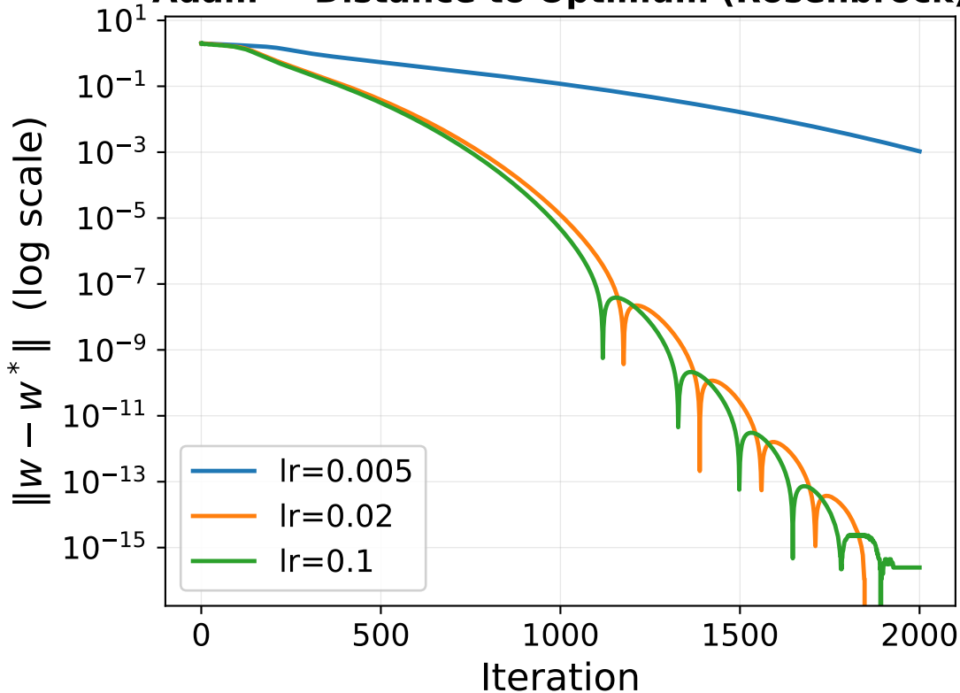
Adam — Distance to Optimum (Rosenbrock)
