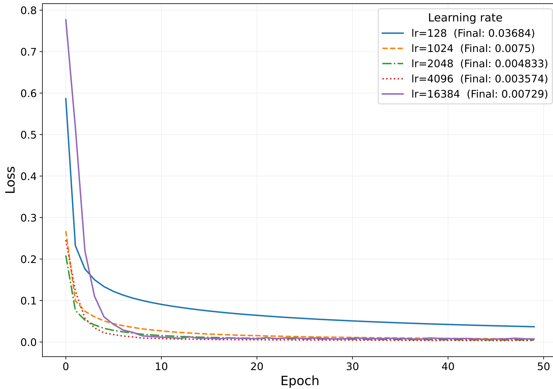
Batch size = 1024
