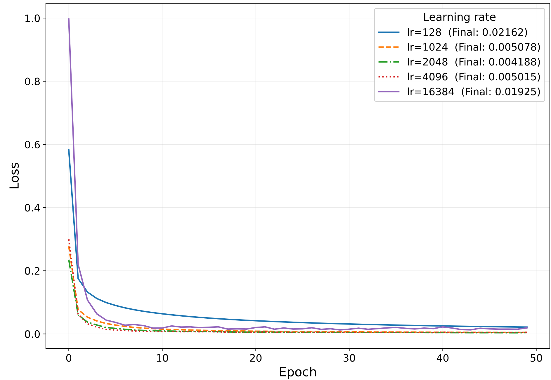
Batch size = 8192
