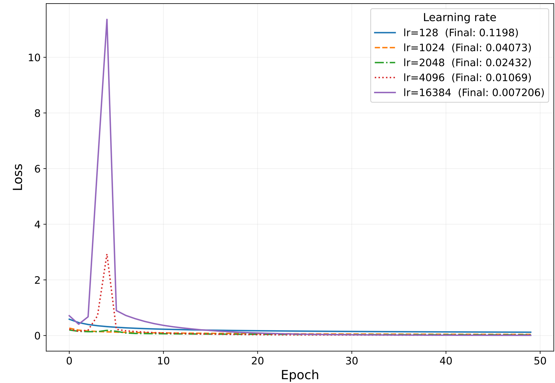
Batch size = 8192
