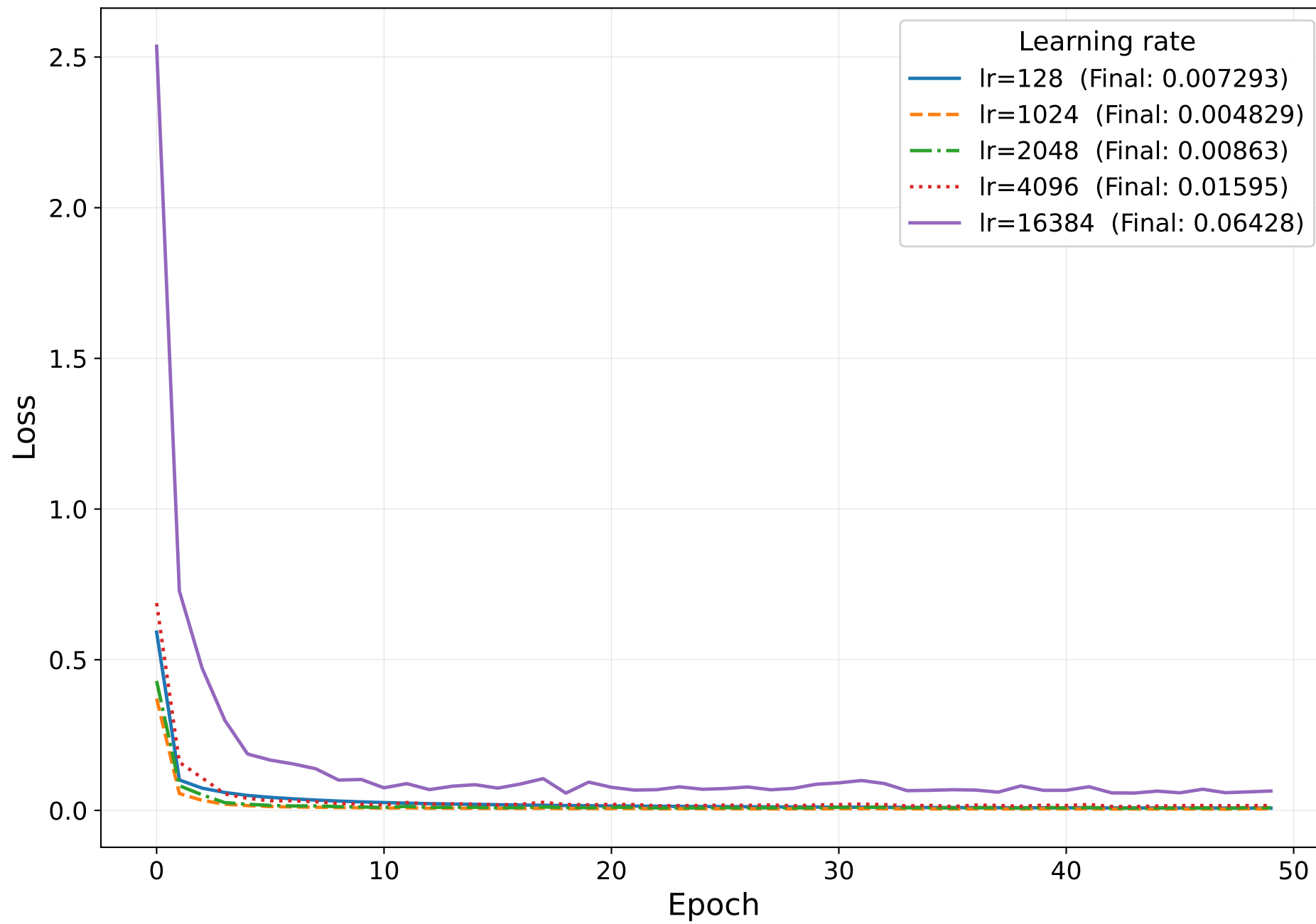
Batch size = 1024
