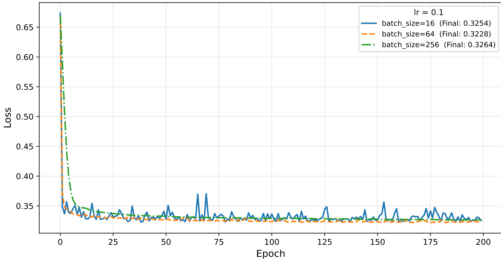
Momentum — Batch Size Sweep (lr=0.1, Logistic (Australian))
