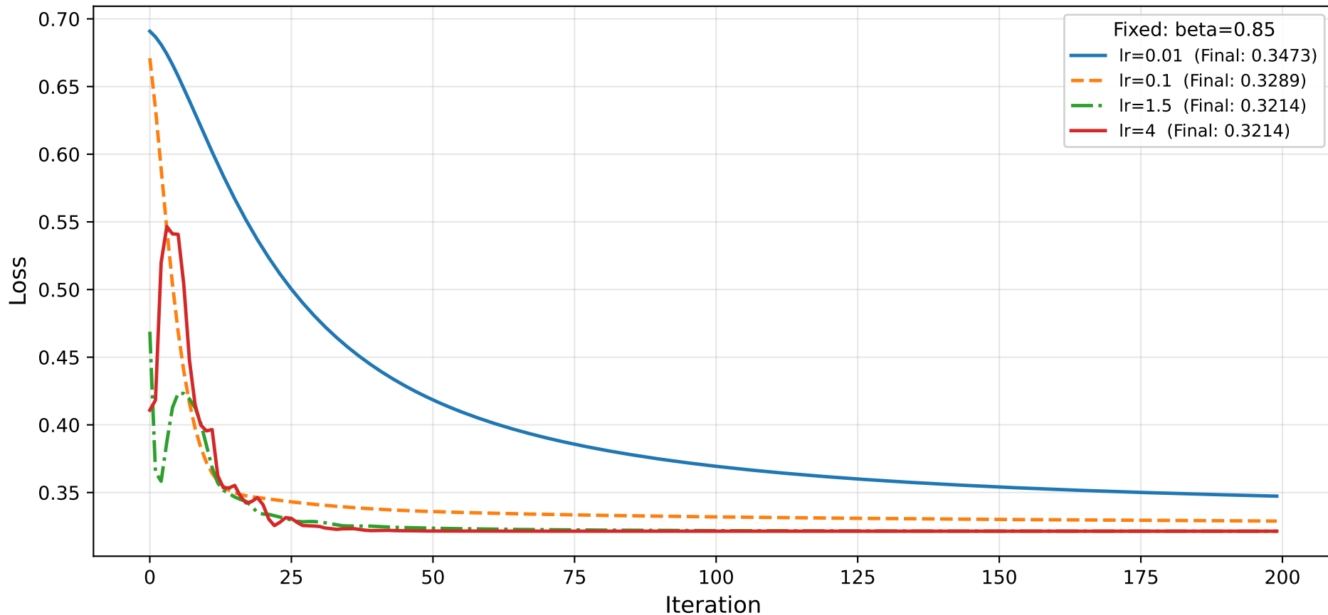
Momentum — LR sweep (Logistic (Australian))
