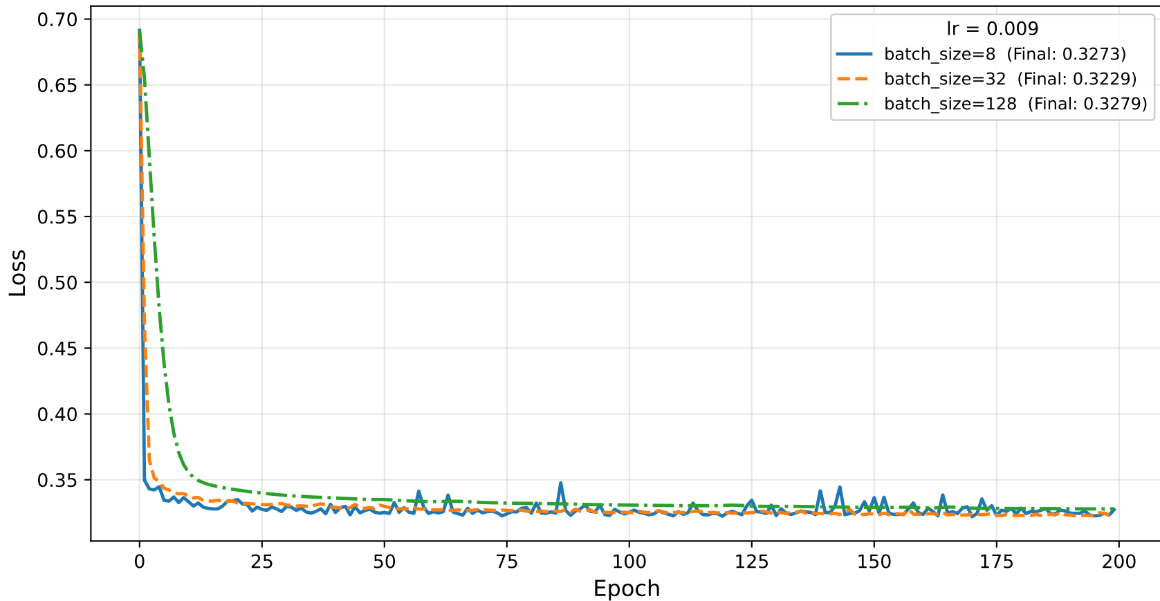
NAG — Batch Size Sweep (lr=0.009, Logistic (Australian))
