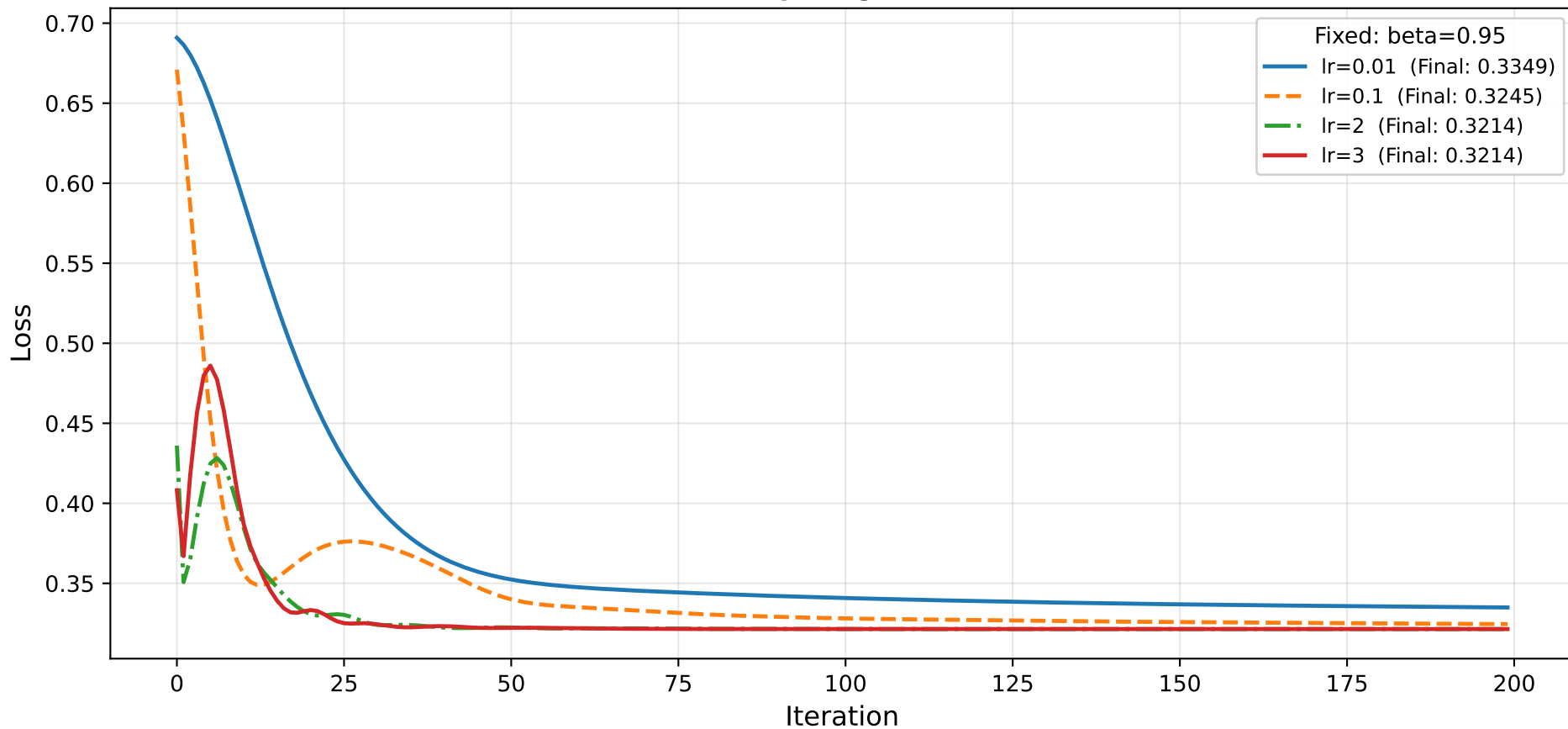
NAG — LR sweep (Logistic (Australian))
