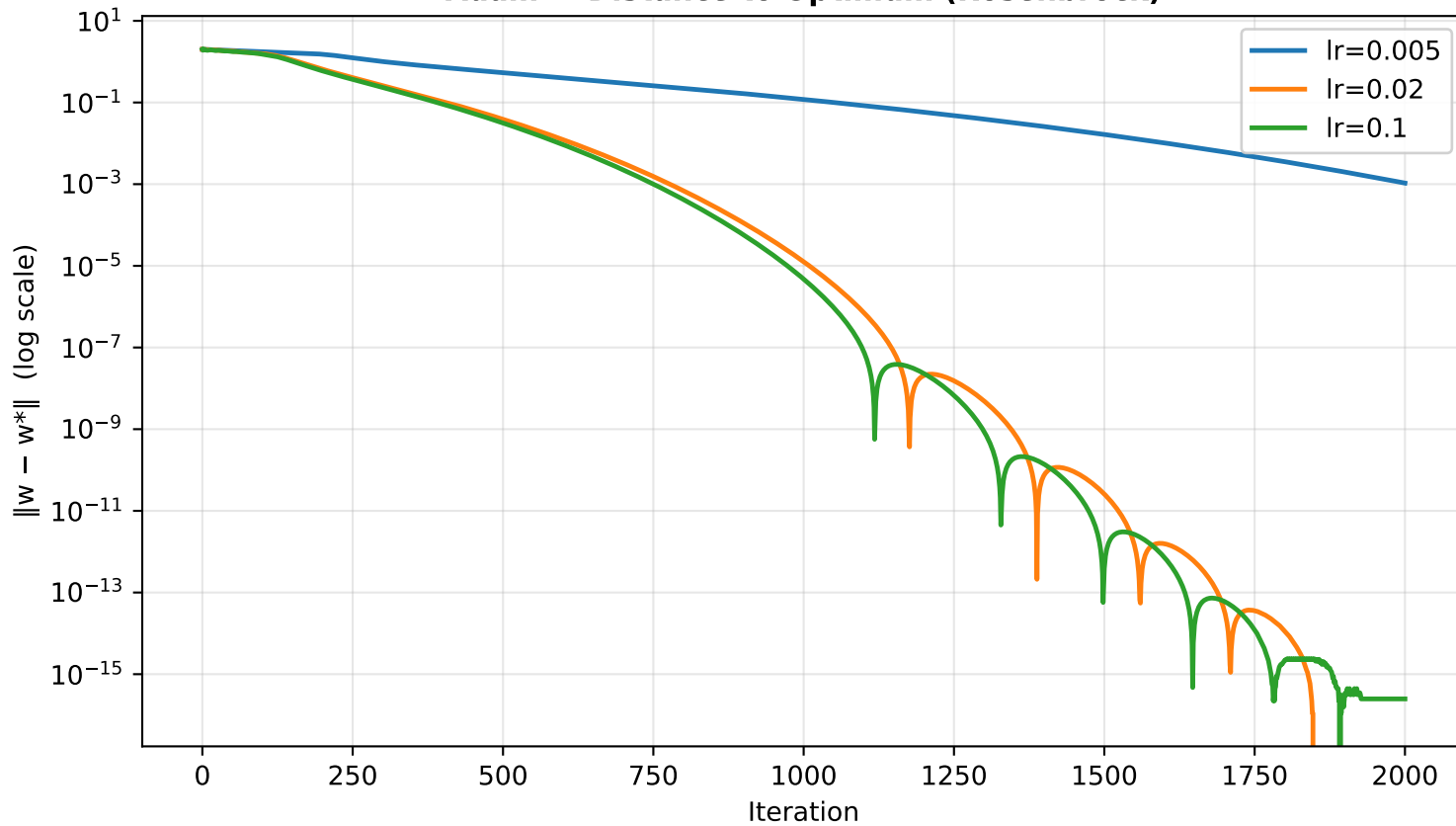
Adam — Distance to Optimum (Rosenbrock)
