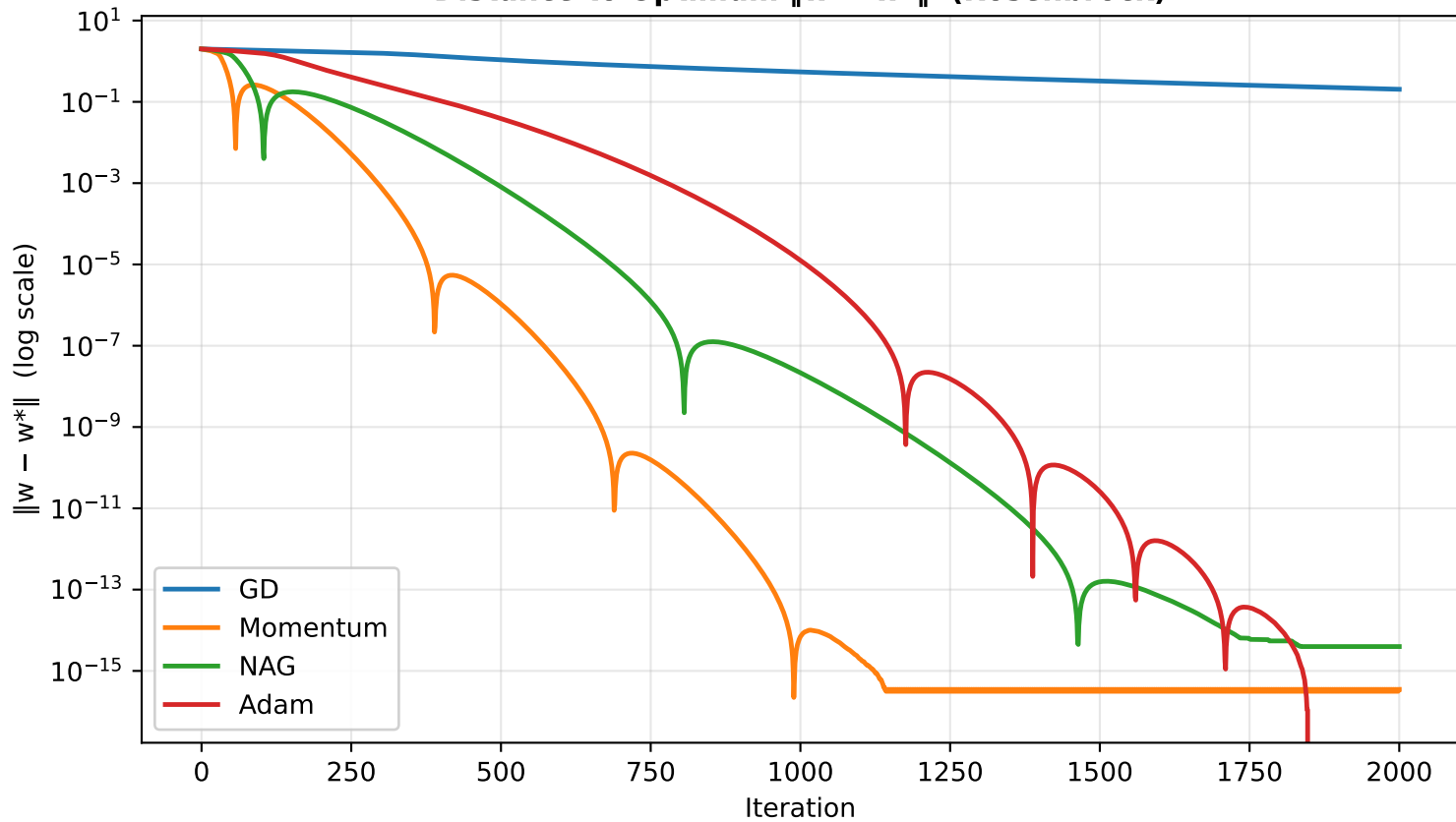
Distance to Optimum \|w - w^*\| (Rosenbrock)
