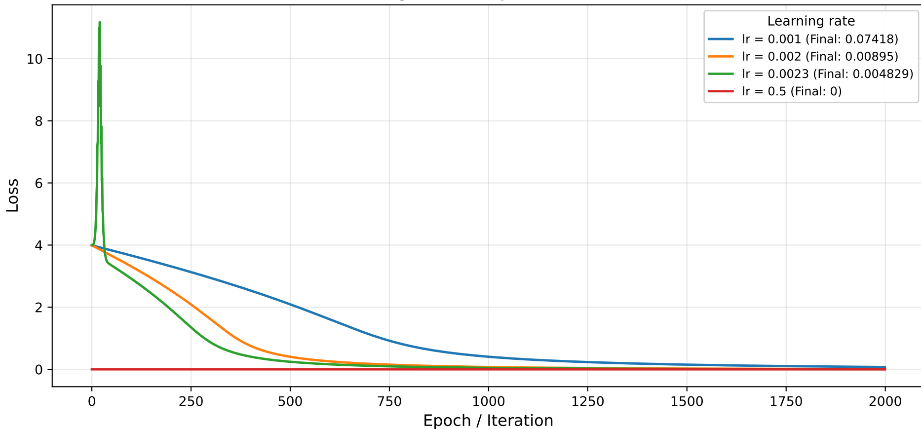
GD - Learning Rate Comparison (Rosenbrock)
