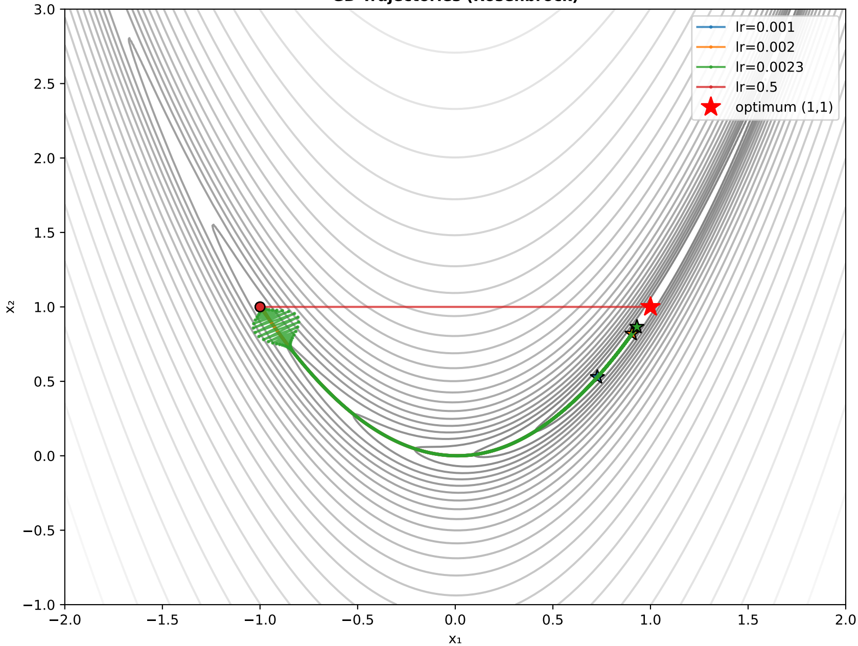
GD Trajectories (Rosenbrock)
