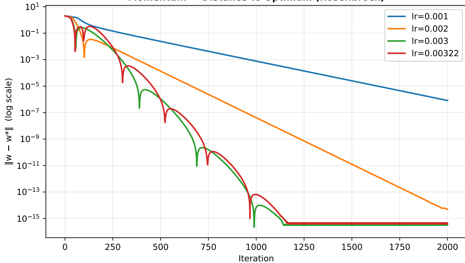
Momentum — Distance to Optimum (Rosenbrock)
