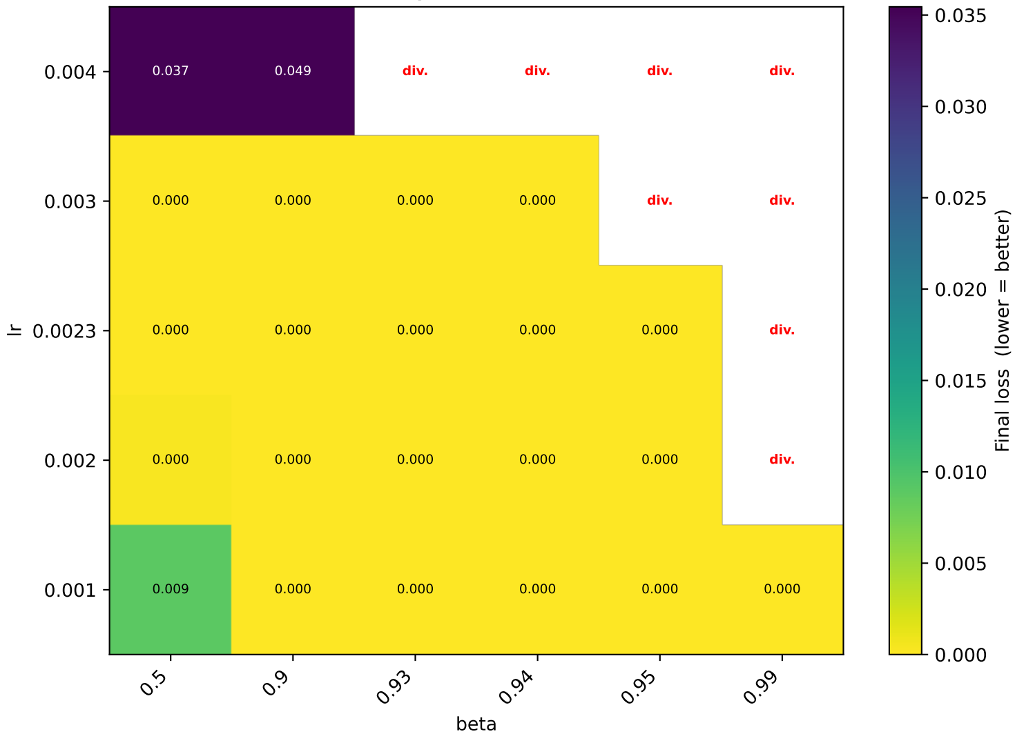
lr × beta Sensitivity — Momentum (Rosenbrock)
