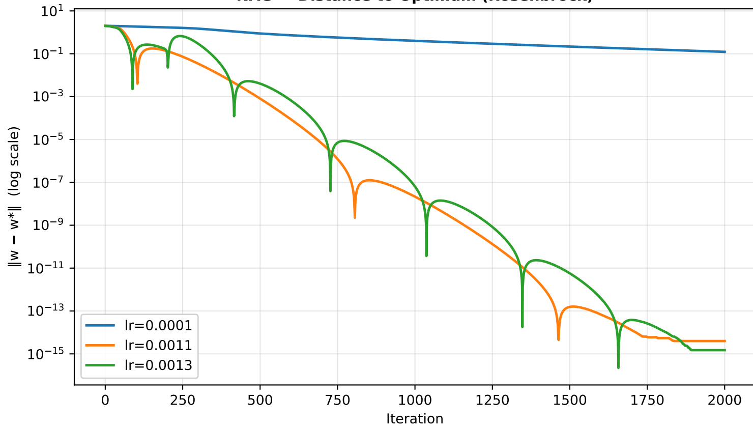
NAG — Distance to Optimum (Rosenbrock)
