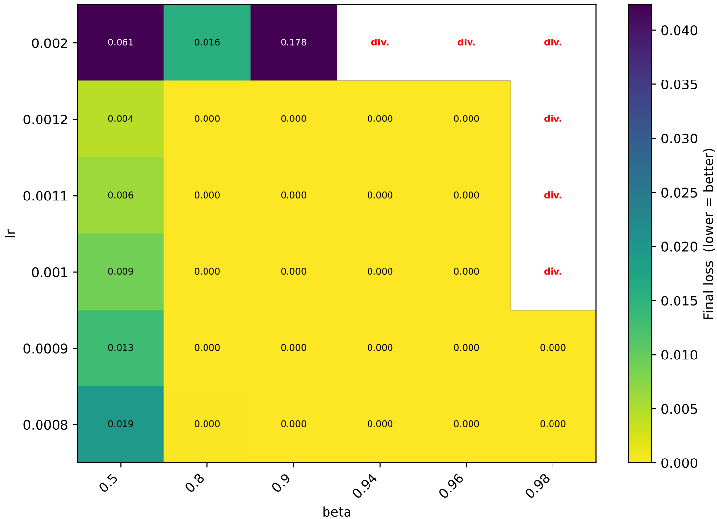
lr × beta Sensitivity — NAG (Rosenbrock)
