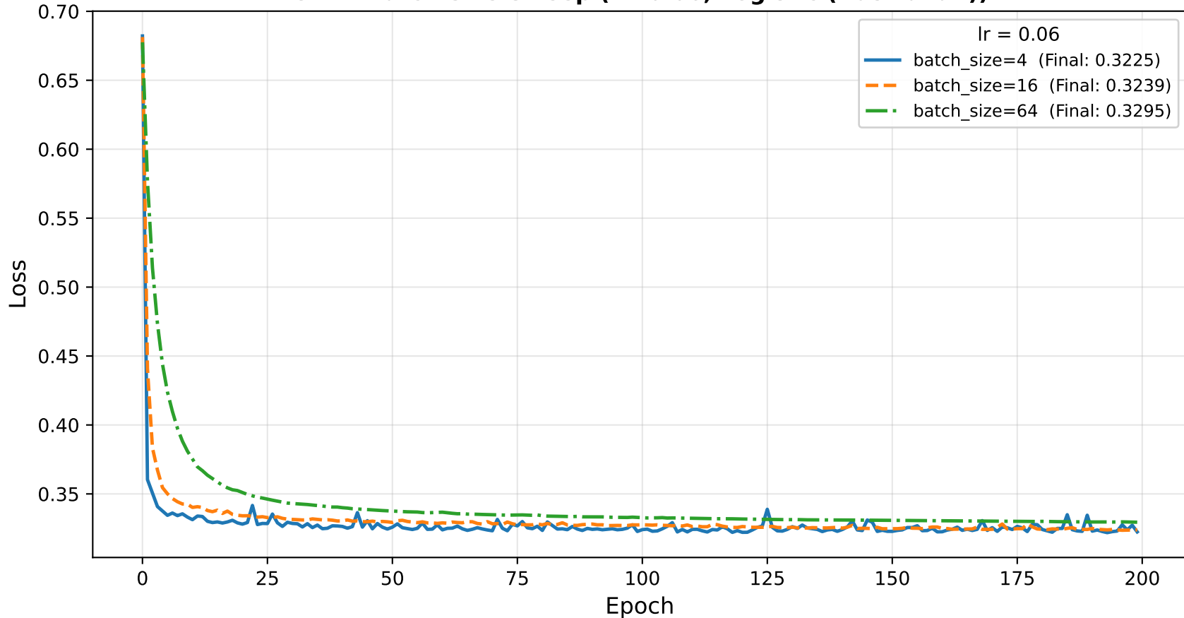
GD — Batch Size Sweep (lr=0.06, Logistic (Australian))
