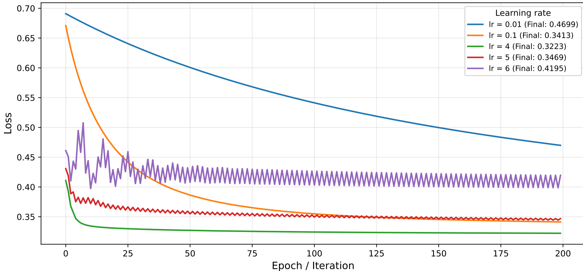
GD — Learning Rate Comparison (Logistic (Australian))
