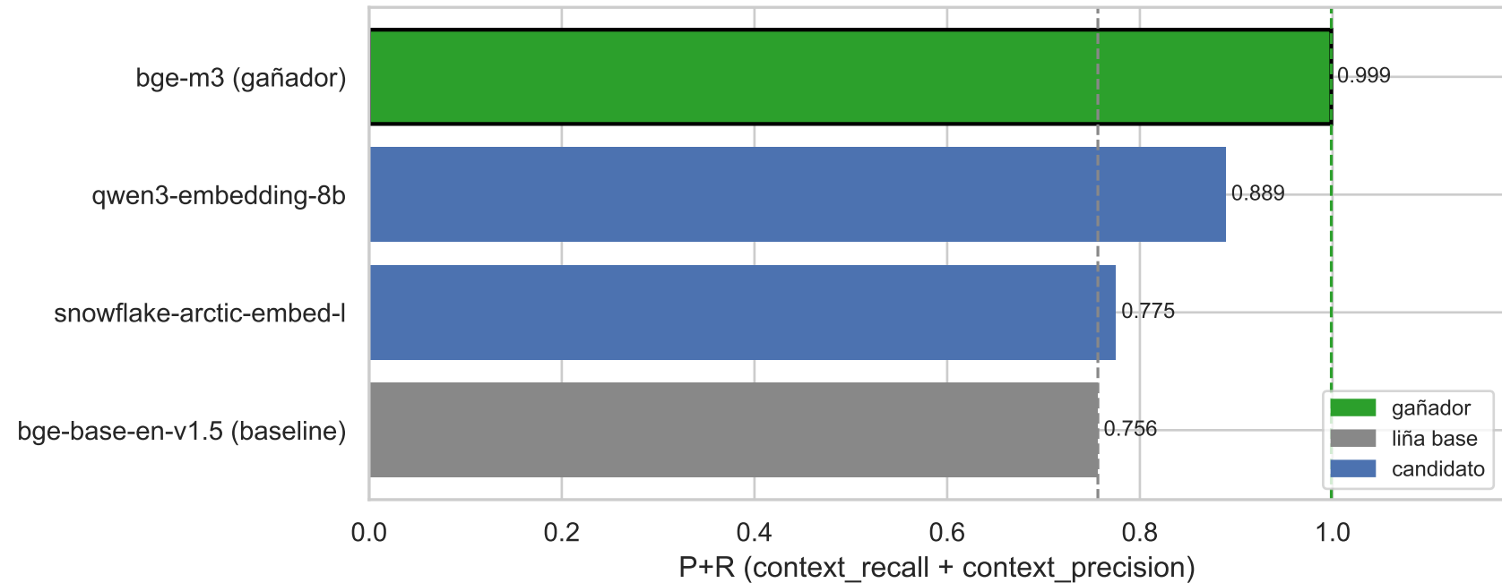
exp1 — Embeddings
