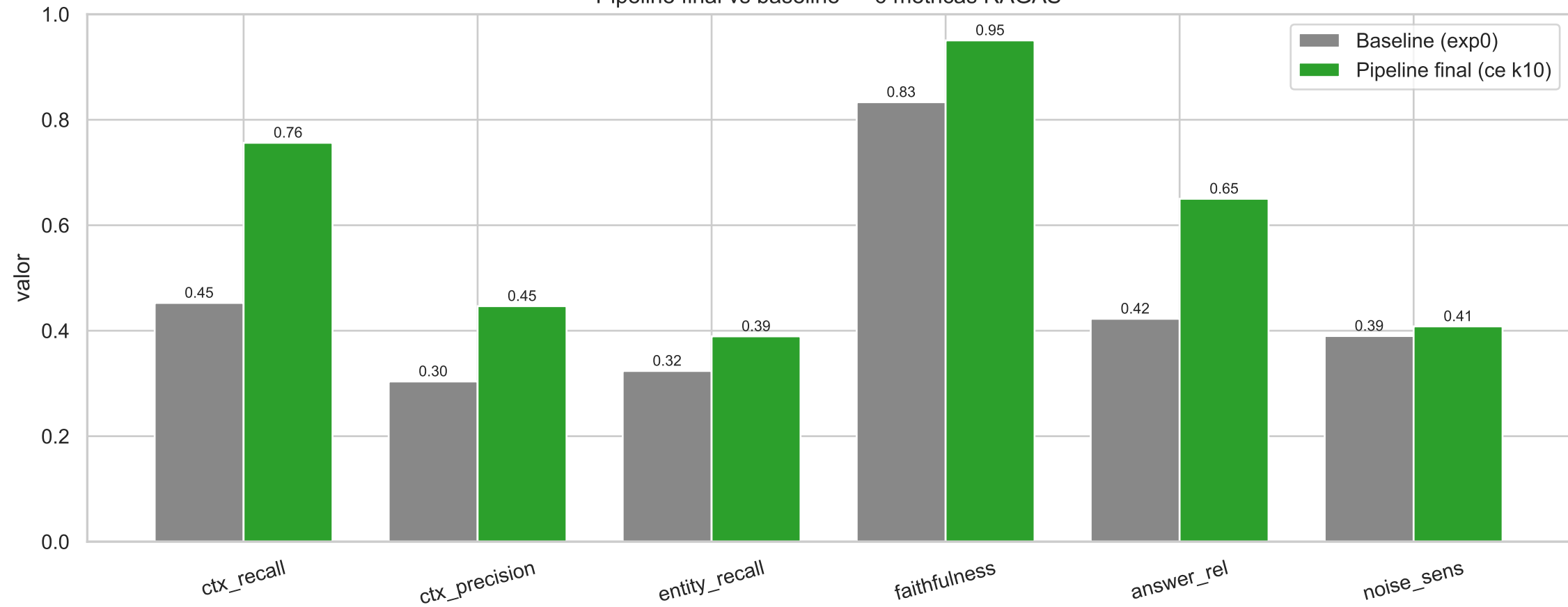
Pipeline final vs baseline — 6 métricas RAGAS
