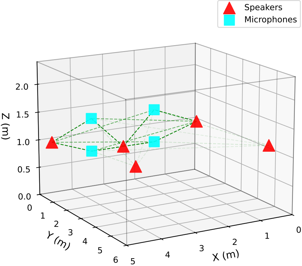
Acoustic Paths 20 Speaker-Mic Pairs
