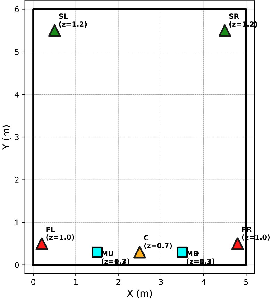
Acoustic Paths 20 Speaker-Mic Pairs
