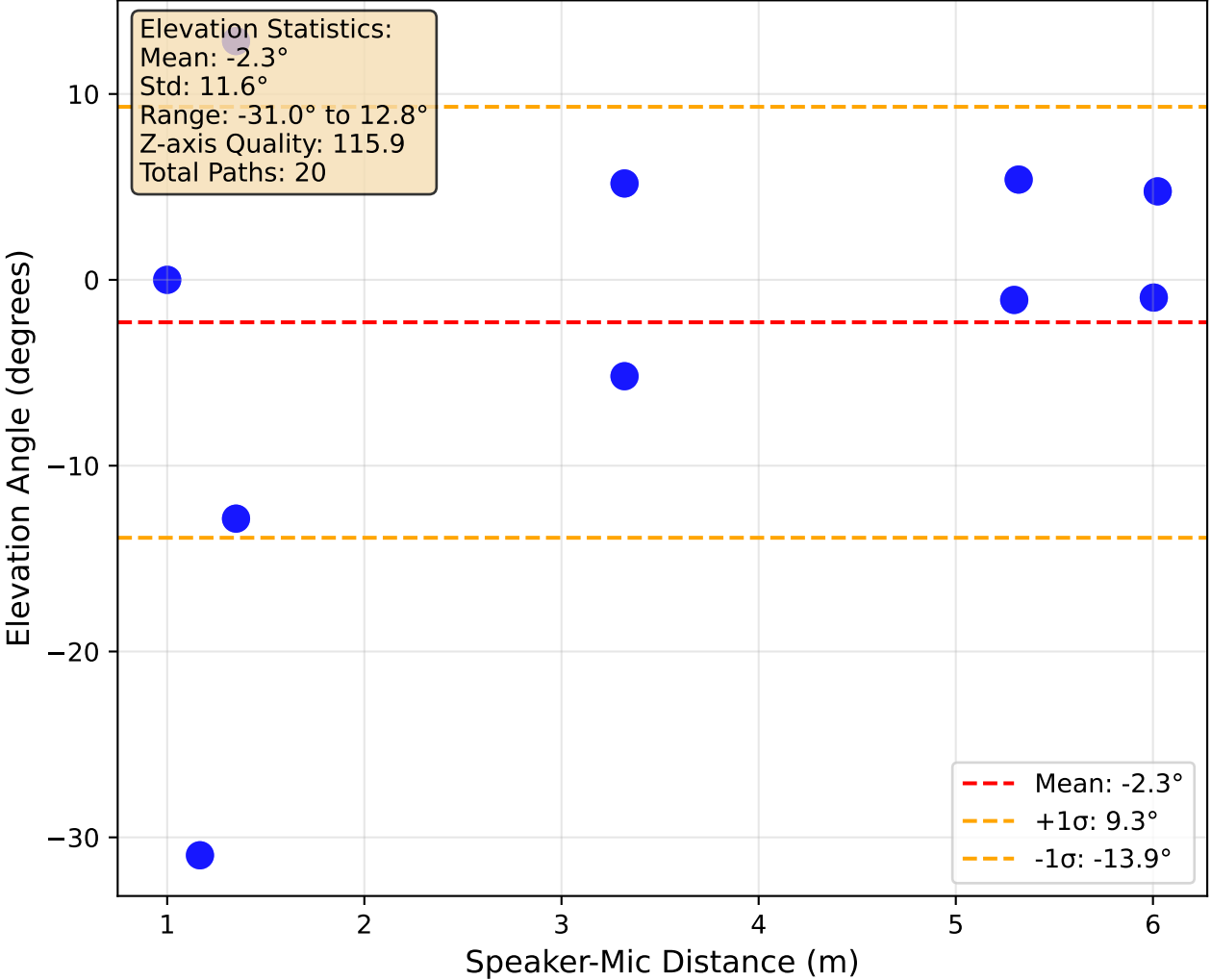
Geometric Quality Analysis Z-Quality: 115.9
