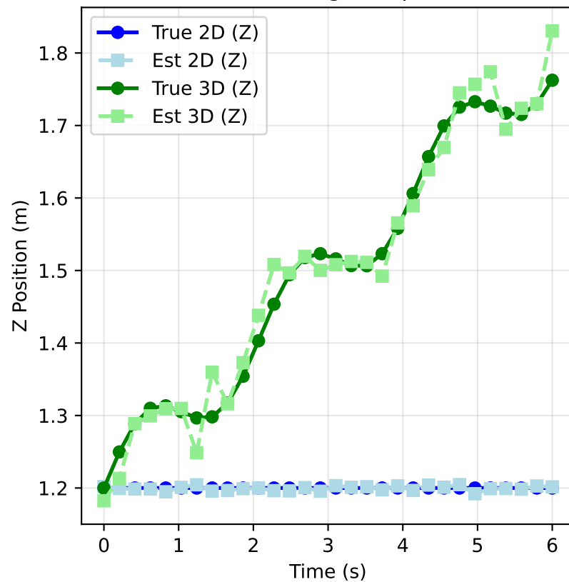
Z-axis Tracking Comparison
