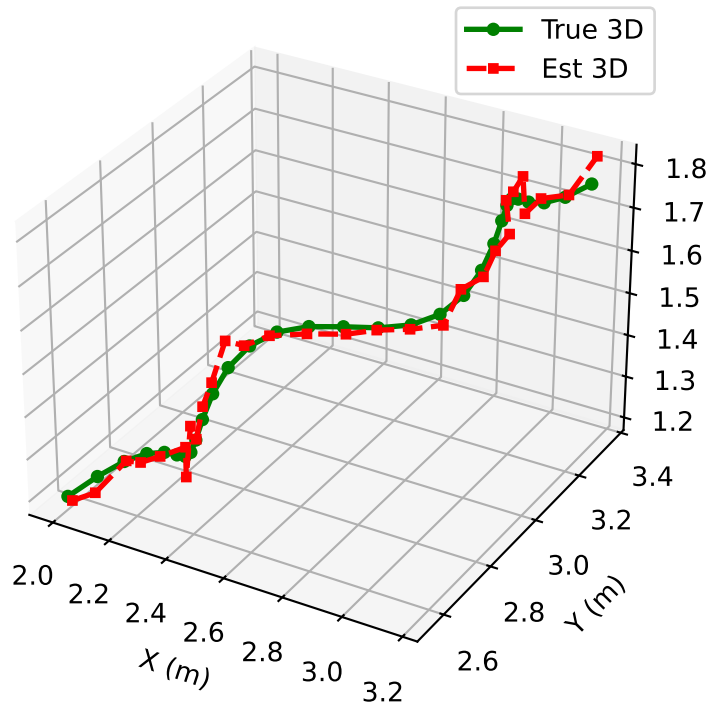
3D Tracking (Full 3D movement)
