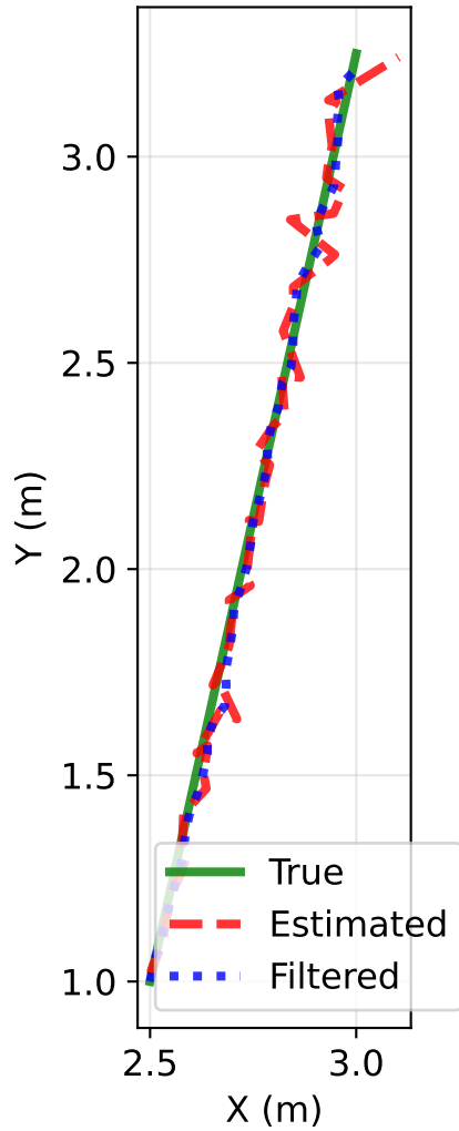
SNR 0 dB - Average XY Trajectory
