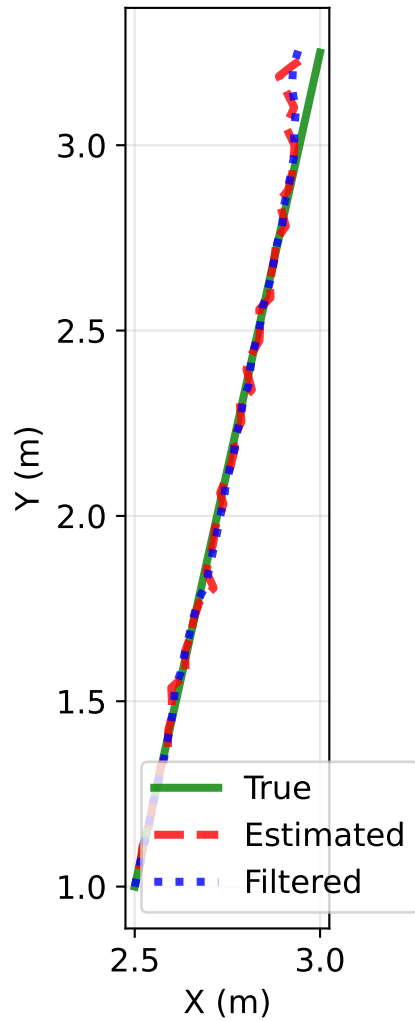
SNR 10 dB - Average XY Trajectory
