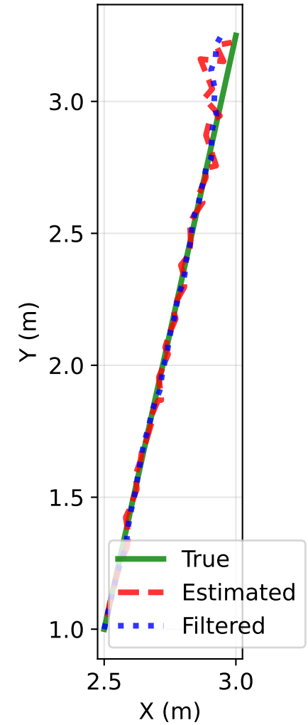
SNR 5 dB - Average XY Trajectory
