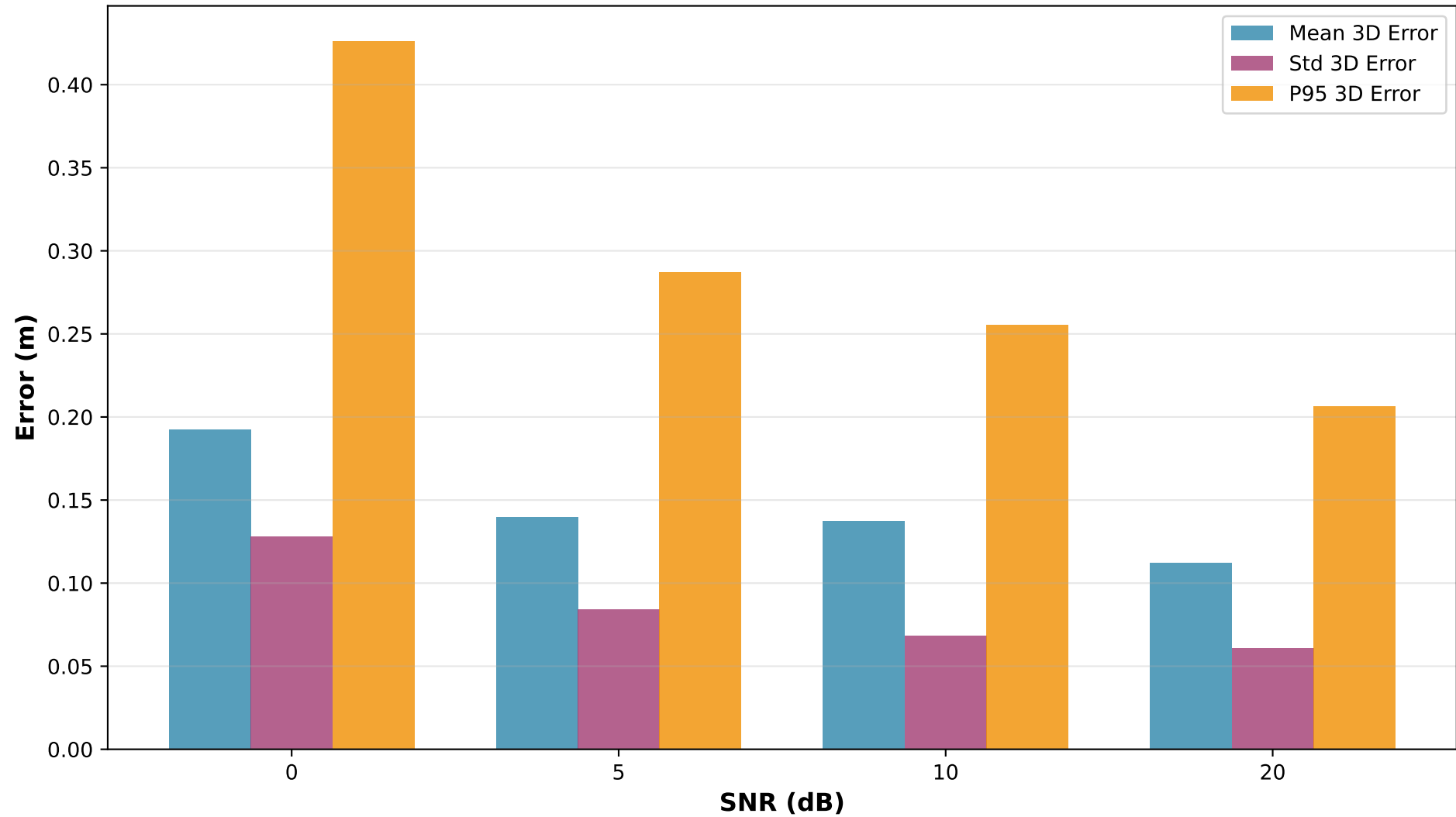
Error Metrics Comparison by SNR Level
