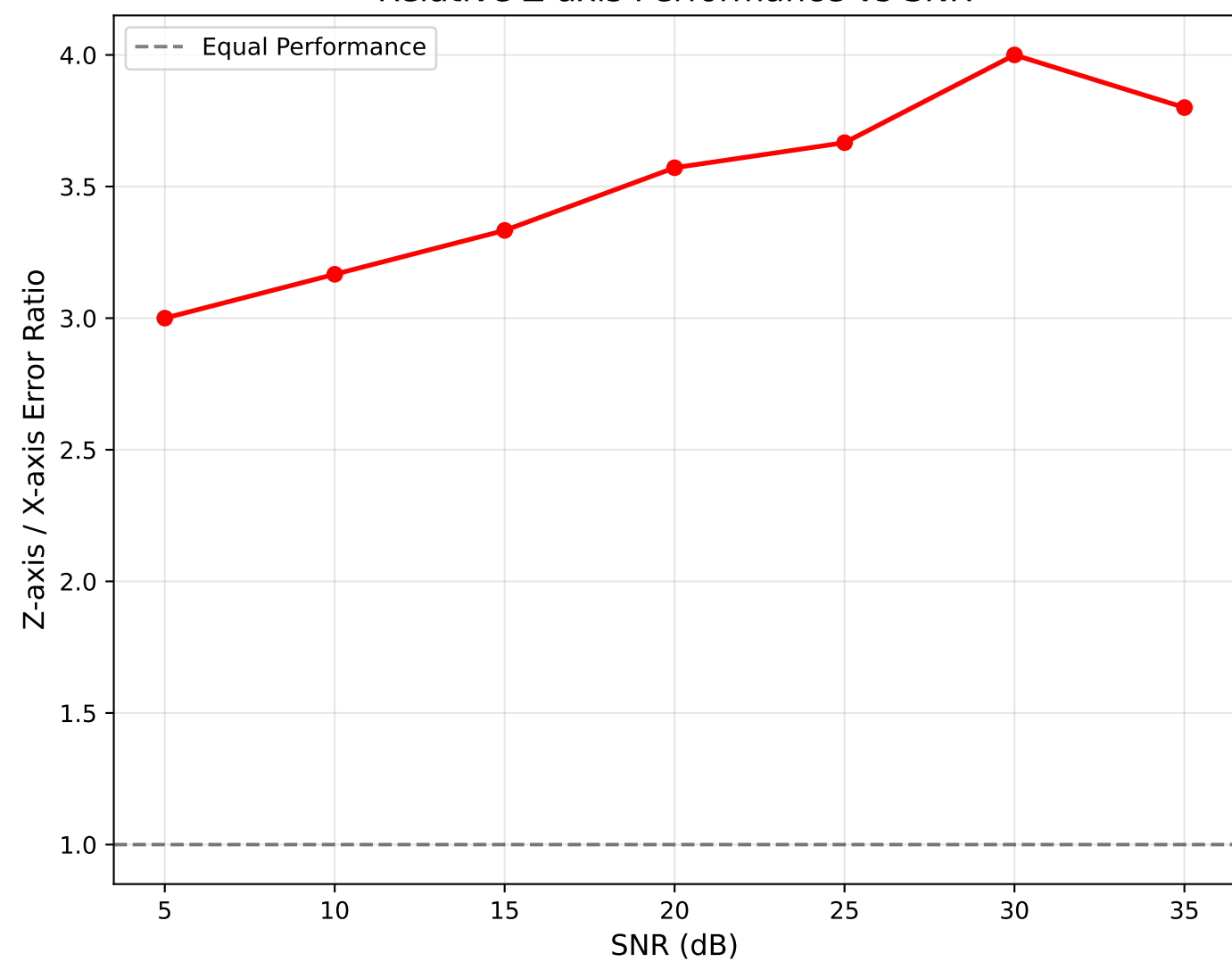
Relative Z-axis Performance vs SNR
