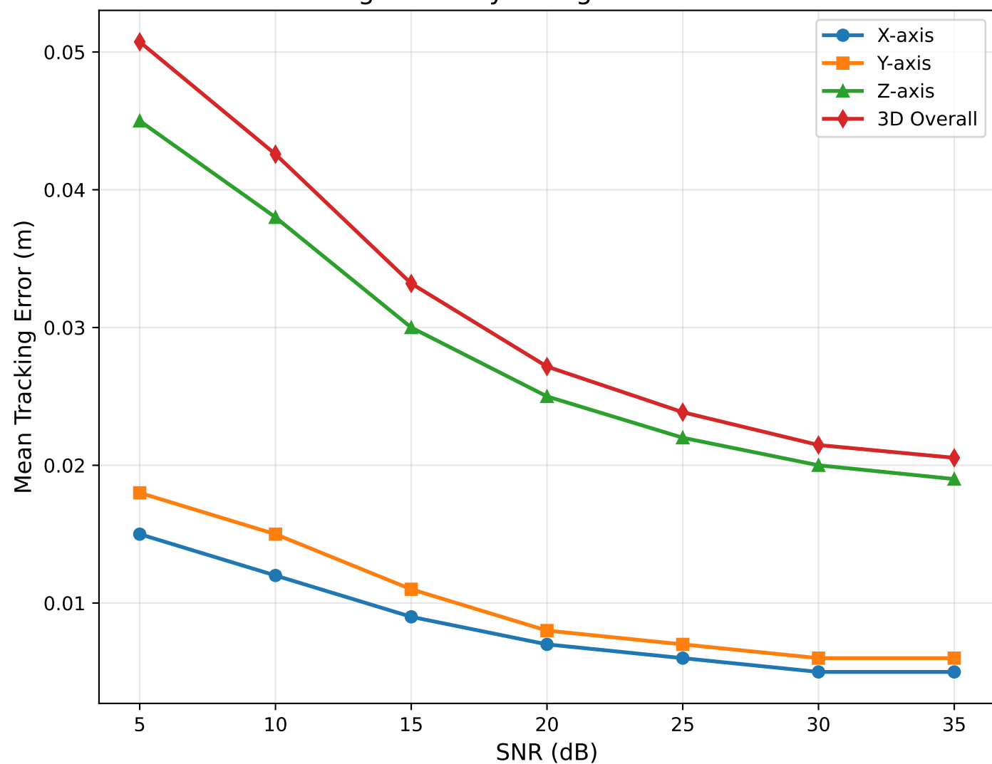
Error Distribution at Different SNR Levels
