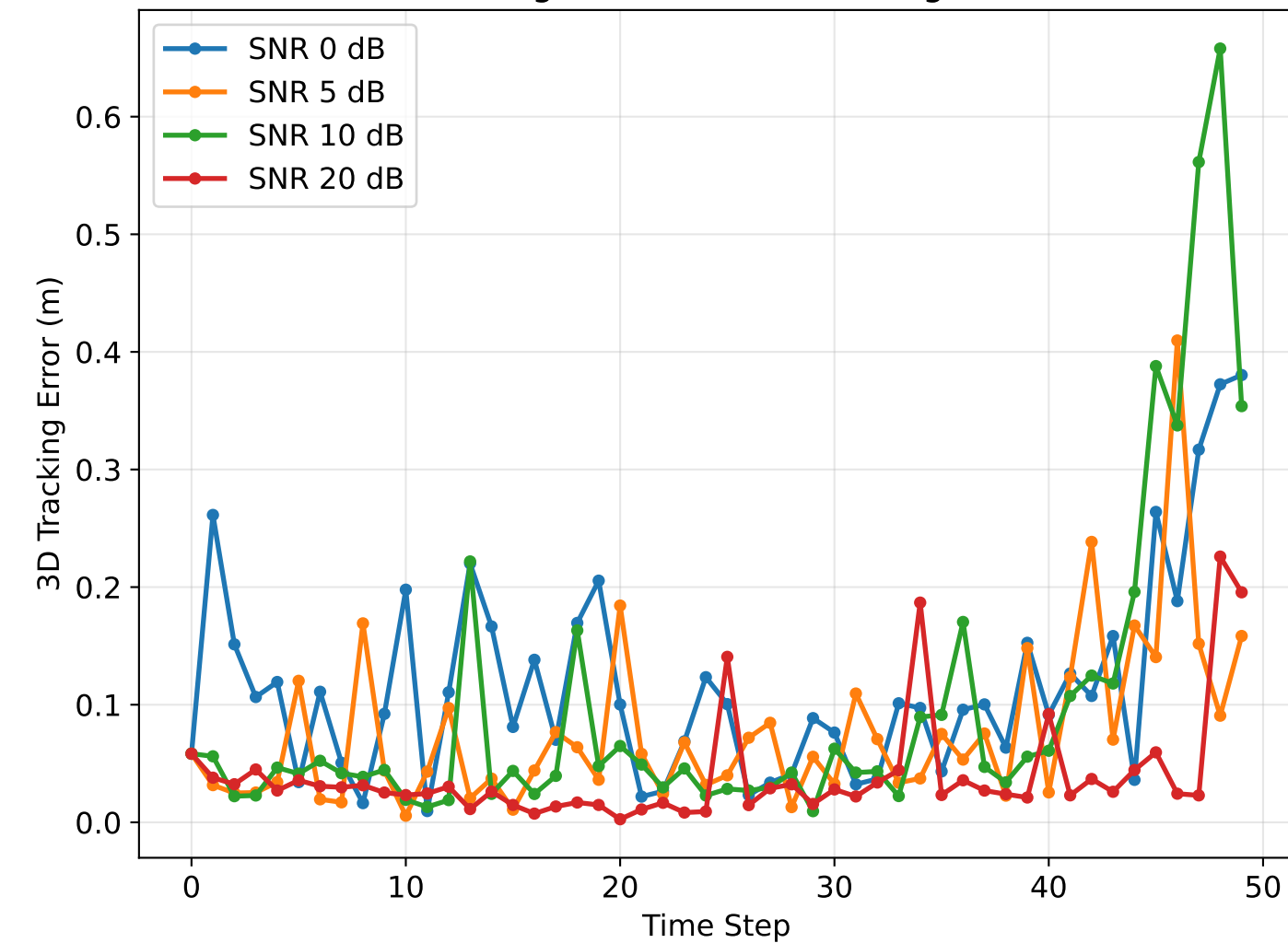
Tracking Error Over Time (Target 0)
