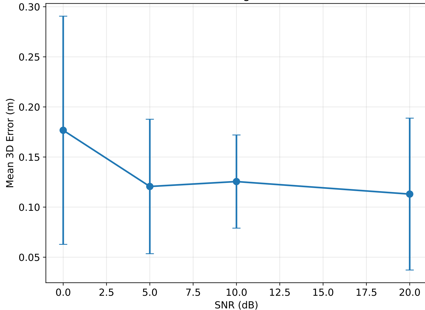
Mean 3D Tracking Error vs SNR
