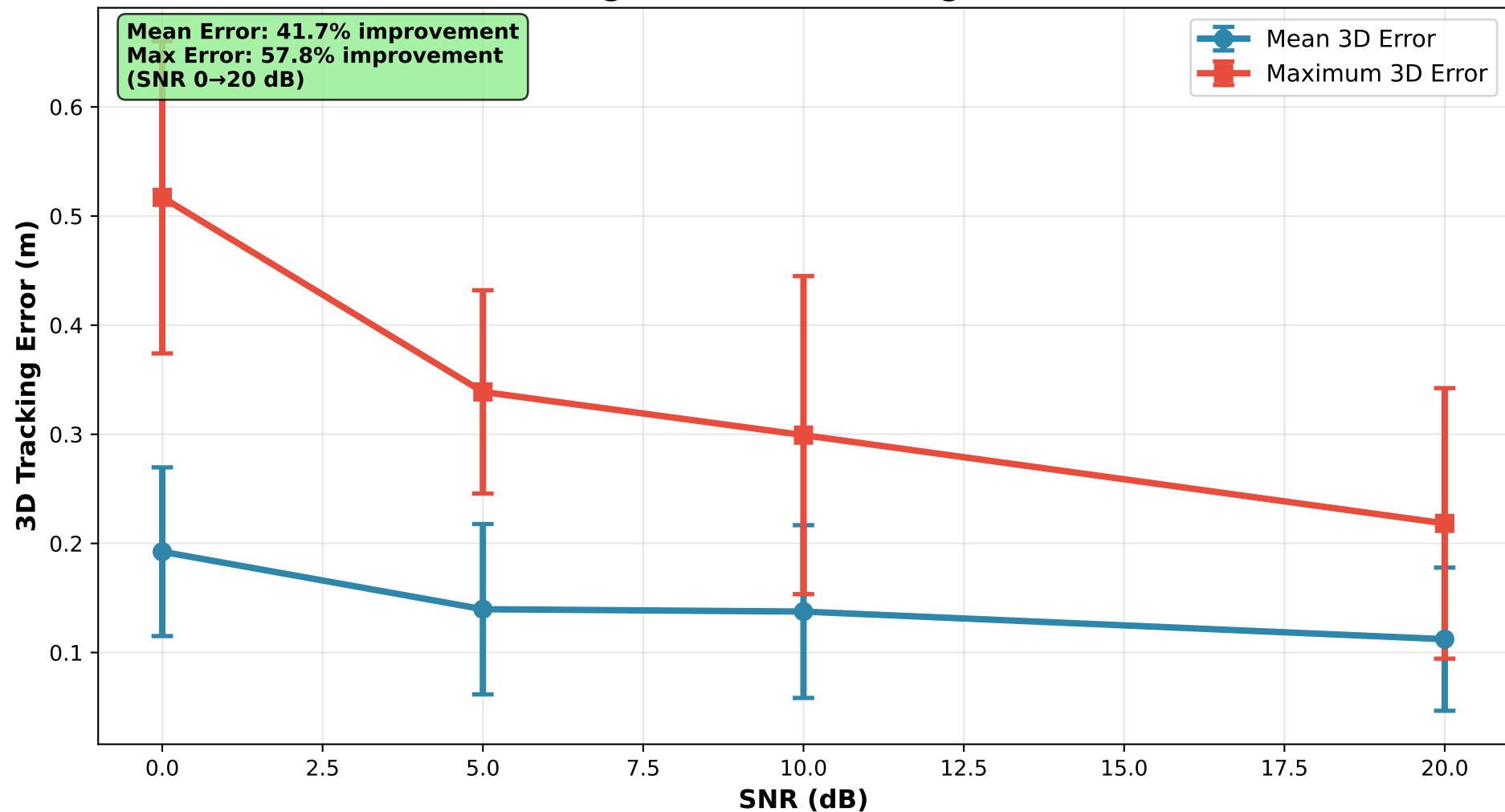
Mean and Maximum 3D Tracking Error vs SNR (Averaged Across All Configurations)
